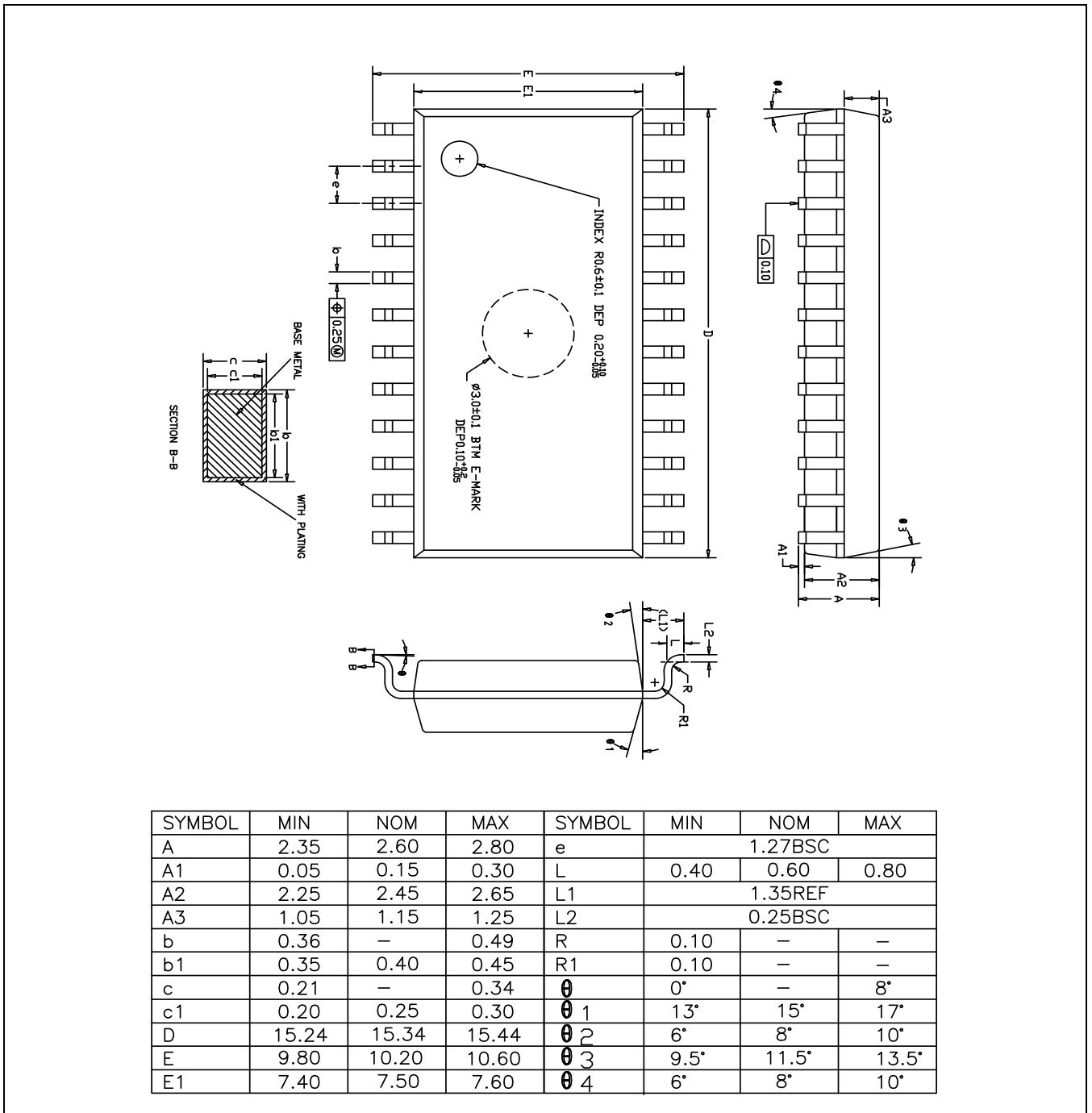
Figure 4-2 SOP24 (1.27mm)封装尺寸
