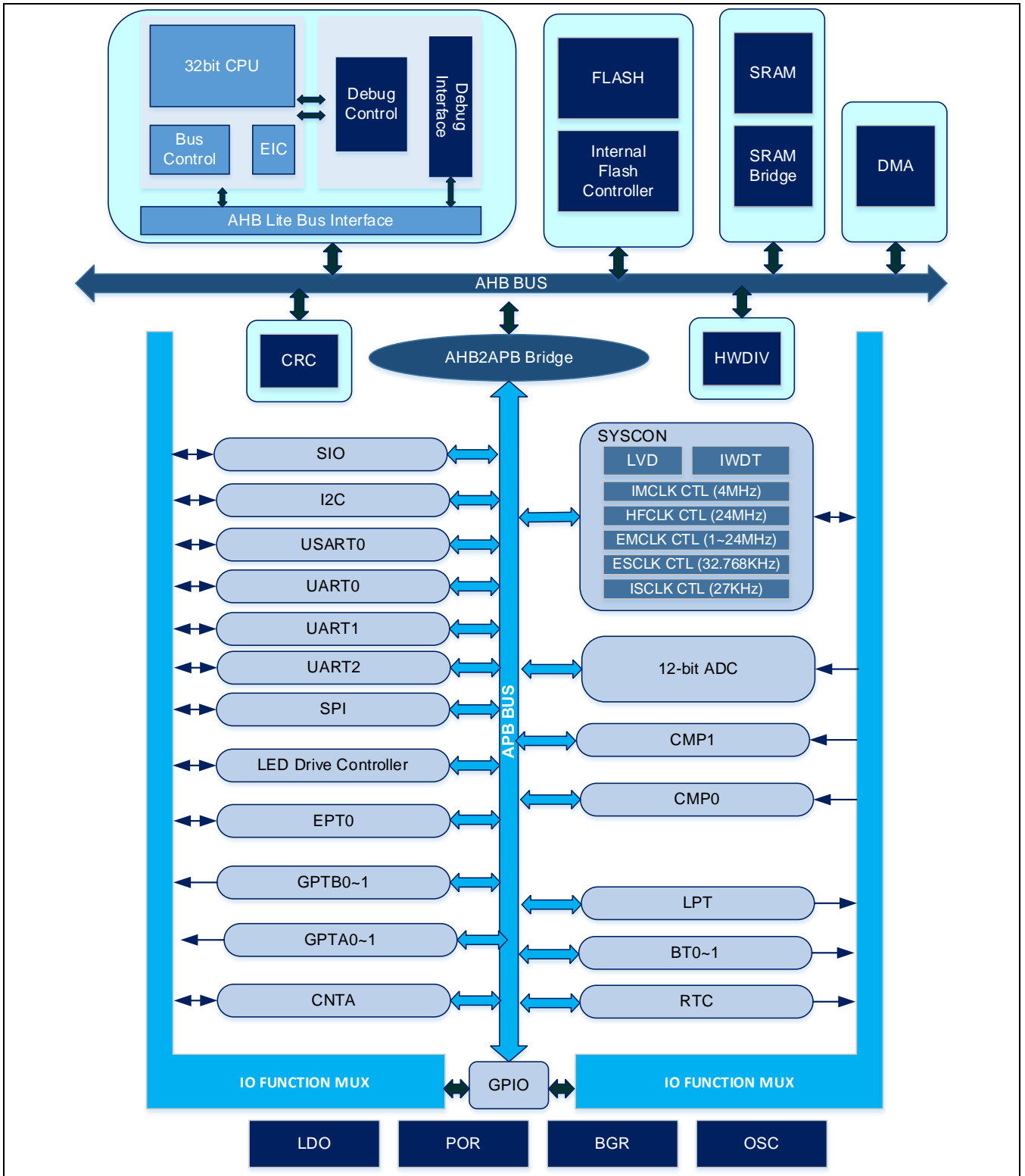
Figure 1-1 APT32F1101模块框图
