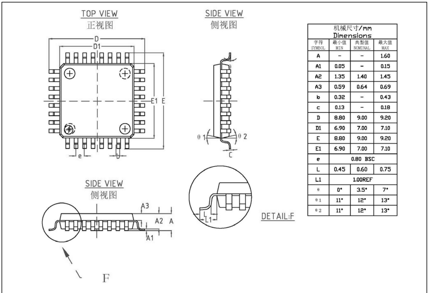
Figure 4-4 32-LQFP (7x7-P0.8mm)封装尺寸
