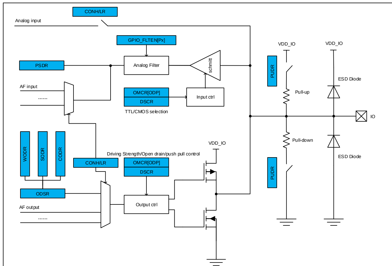
Figure 10-1 GPIO原理图
