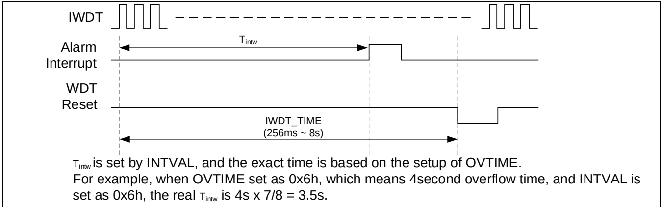
Figure 7-10 IWDT 计数器溢出和报警中断
