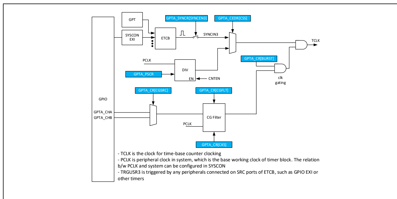
Figure 12-2 时钟控制模块
