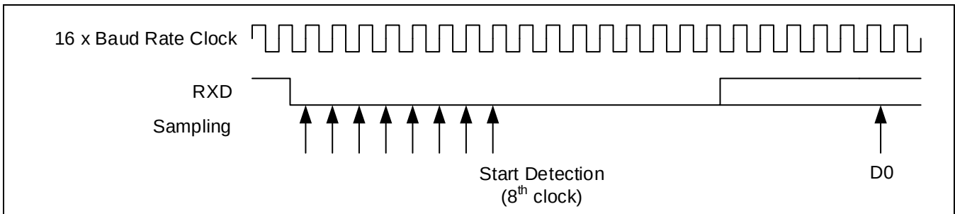
Figure 16-2 起始位检测
