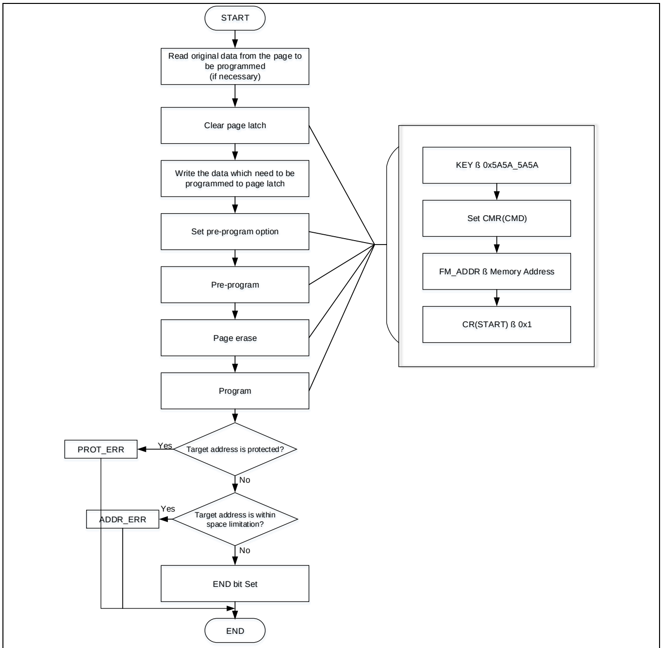
Figure 6-6 Flash Write – Normal Mode
