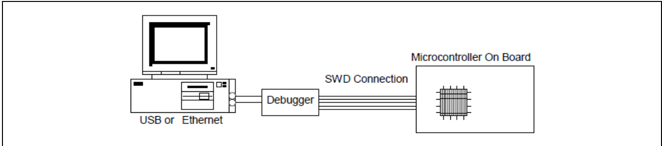
Figure 6-4 通过调试接口的烧写
