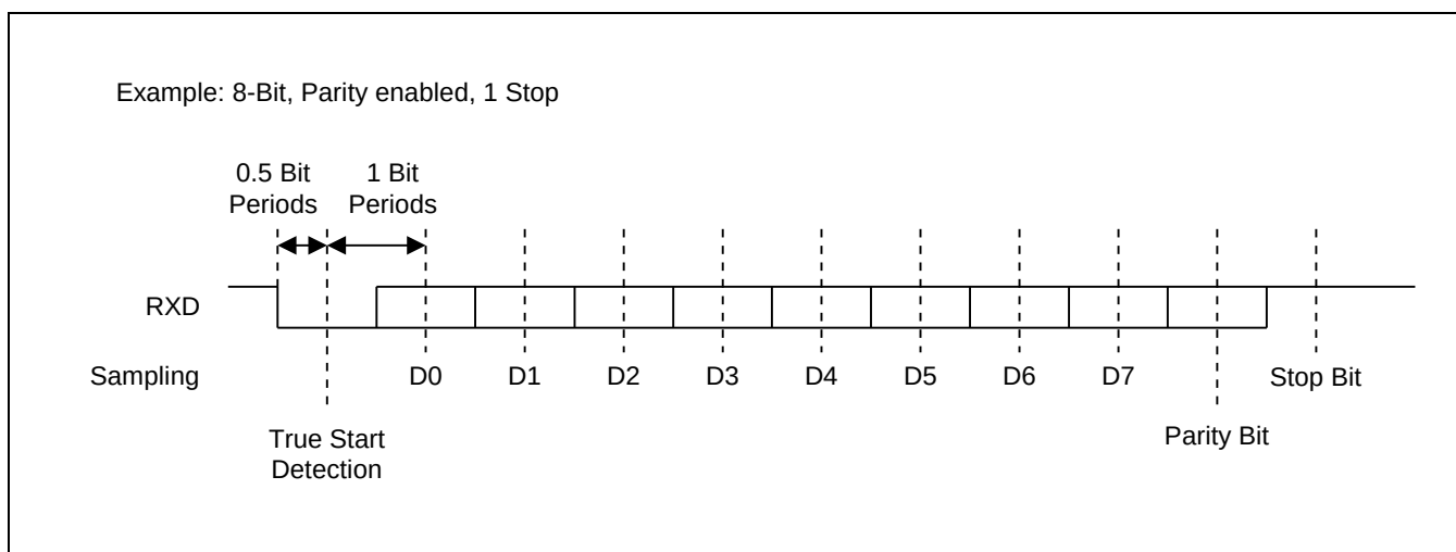
Figure 17-4 异步模式, 字节接收
