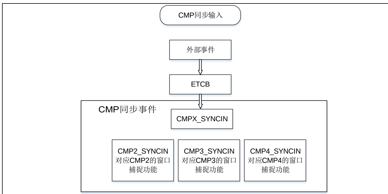
Figure 18-8 同步触发
