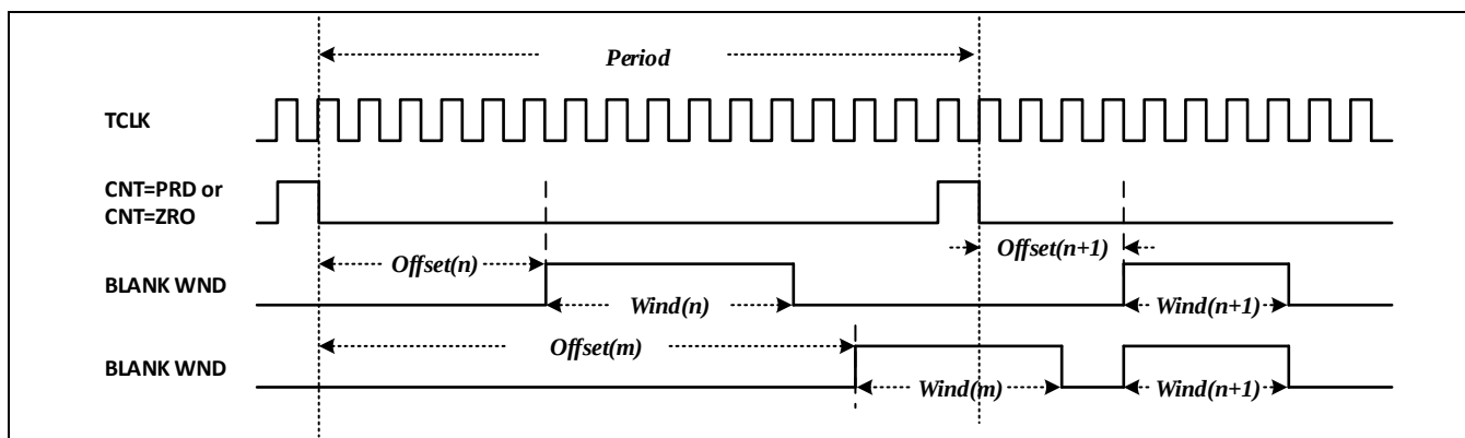
Figure 13-43 滤波器时序
