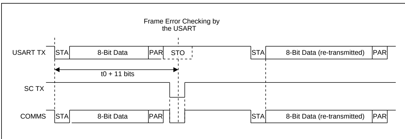
Figure 17-8 Smart-Card 发送错误
