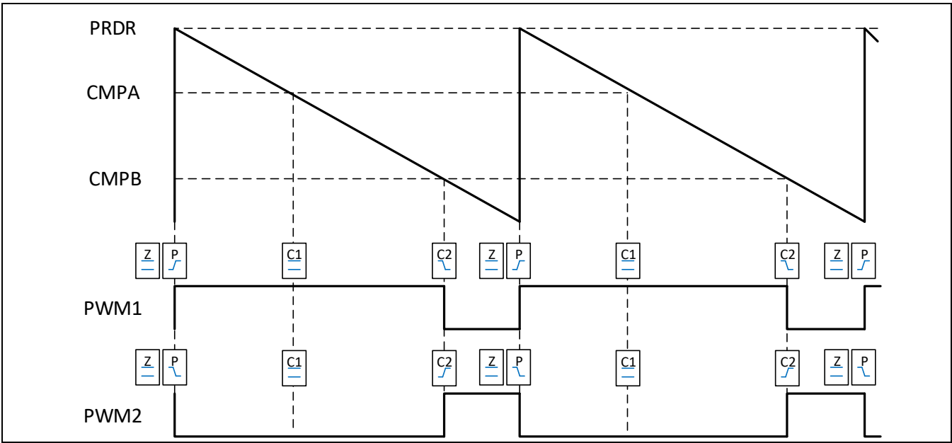
Figure 13-18 递减单沿，非对称波形输出
