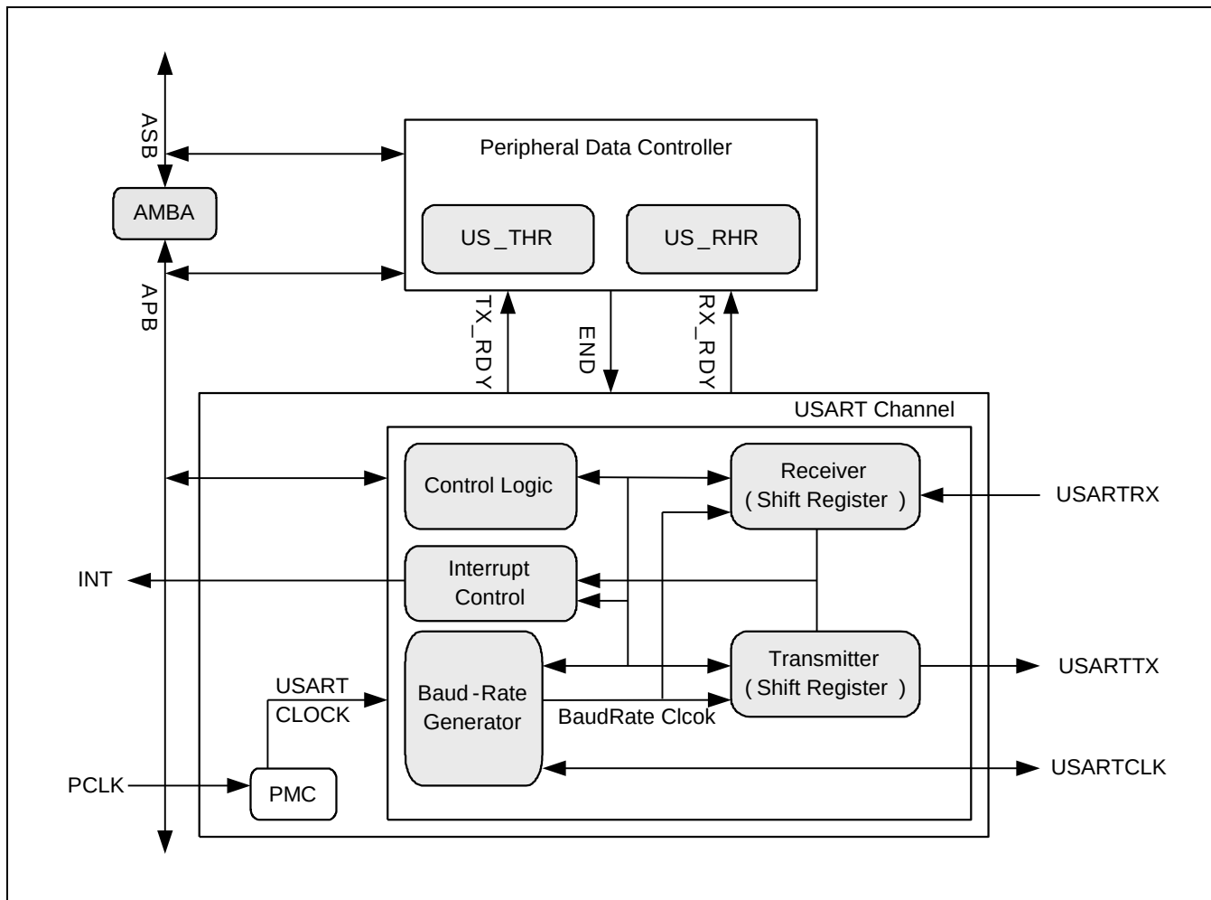
Figure 17-1 USART模块框图
