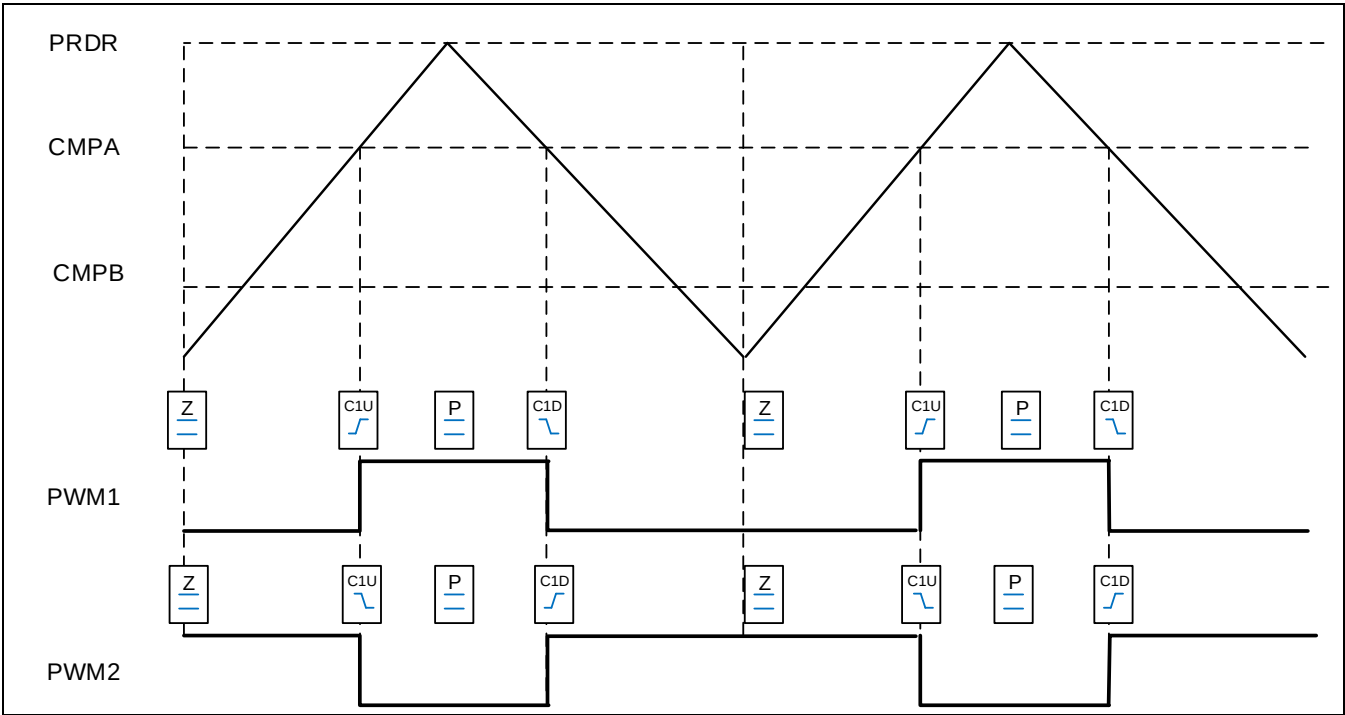
Figure 13-19 递增递减，双沿对称波形输出
