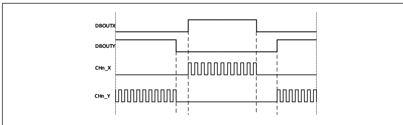
Figure 13-32 简单的斩波输出
