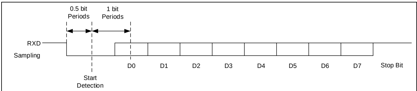
Figure 16-3 接收数据
