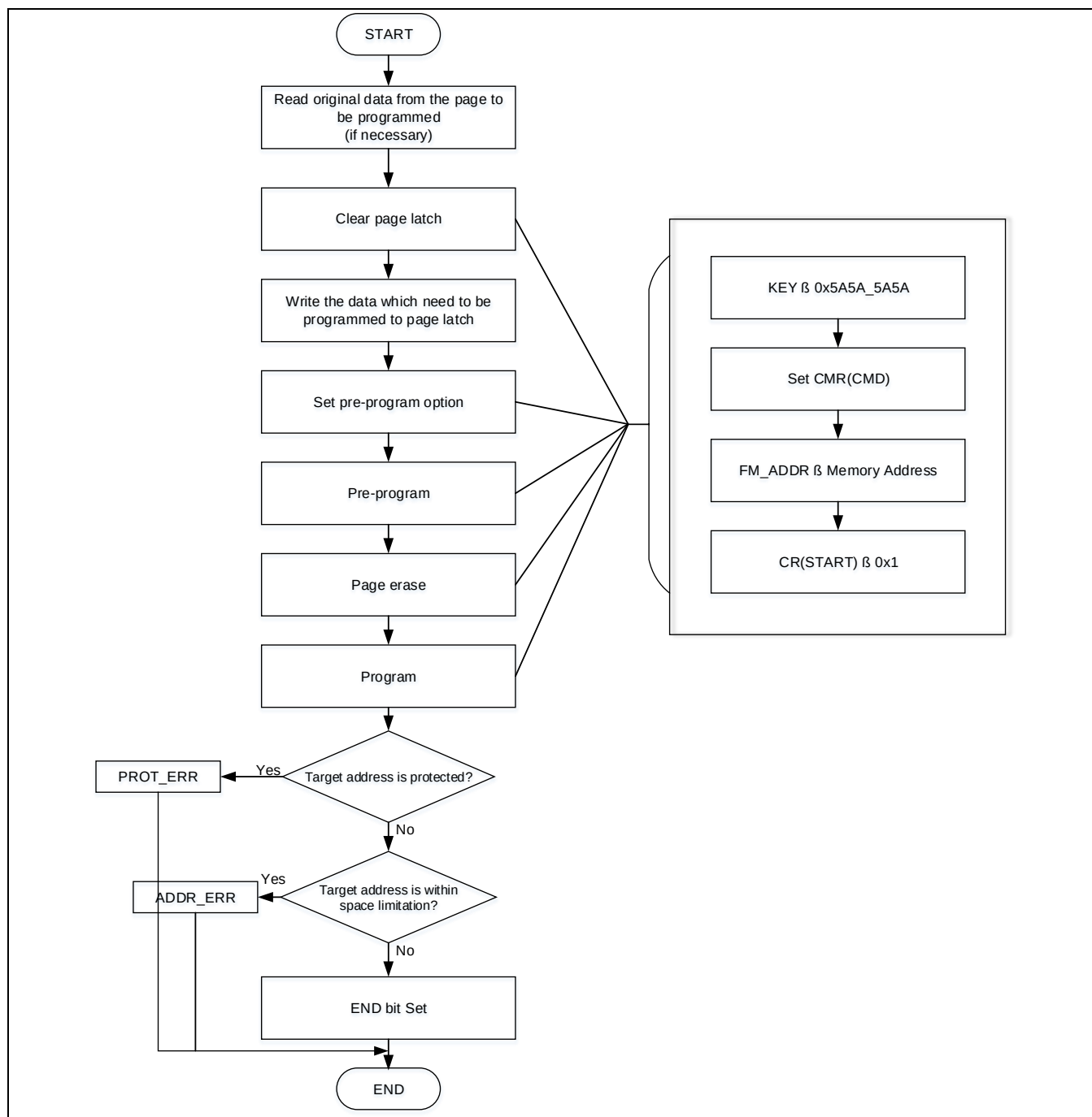
Figure 6-7 Flash Write – Parallel Mode
