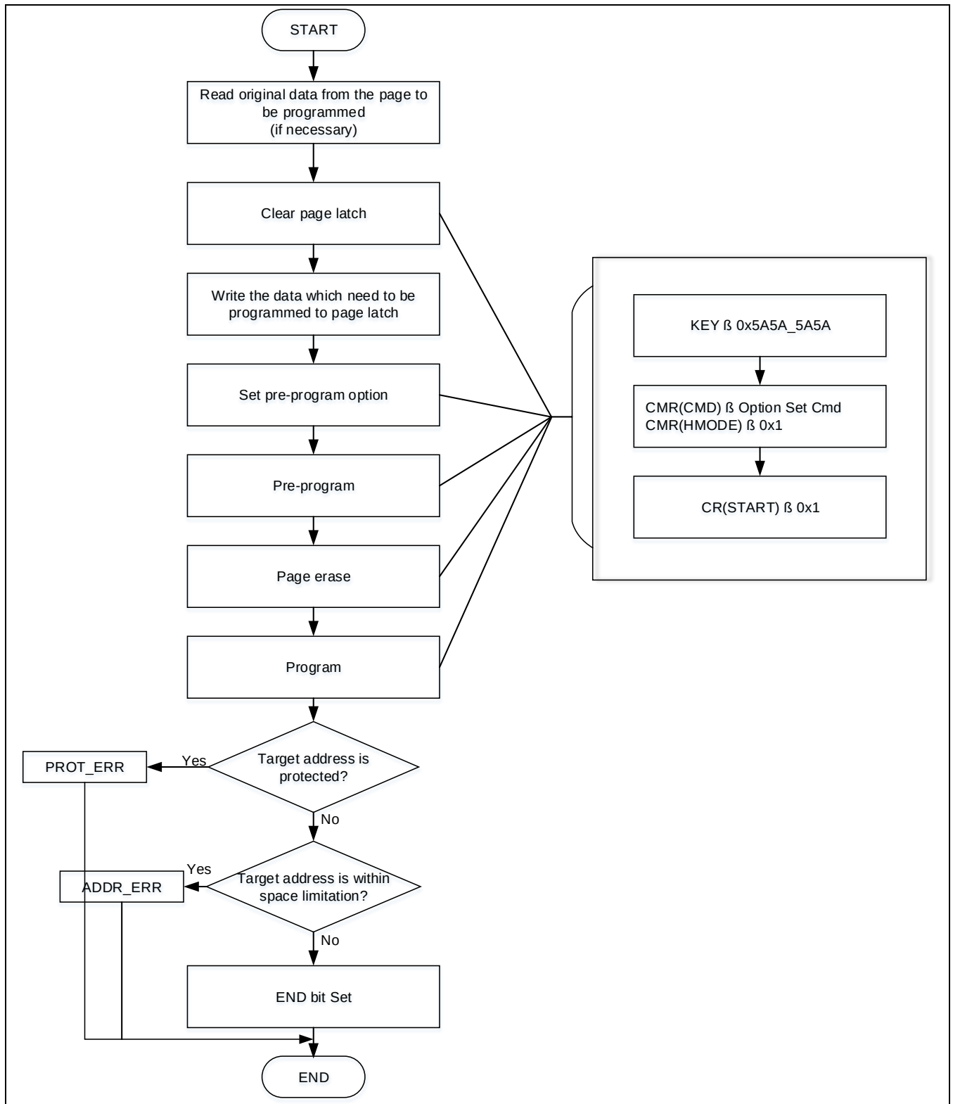
Figure 6-10 Option Cells Write
