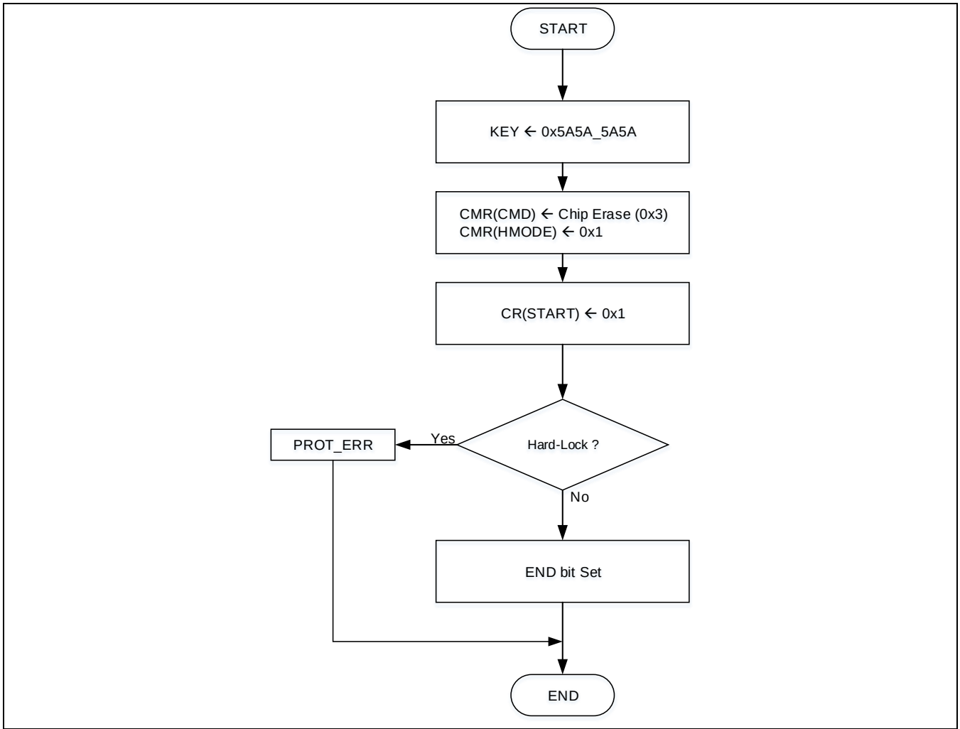
Figure 6-9 Chip Erase
