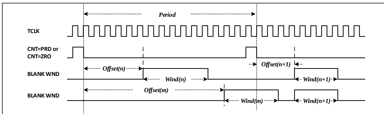
Figure 12-29 滤波器时序
