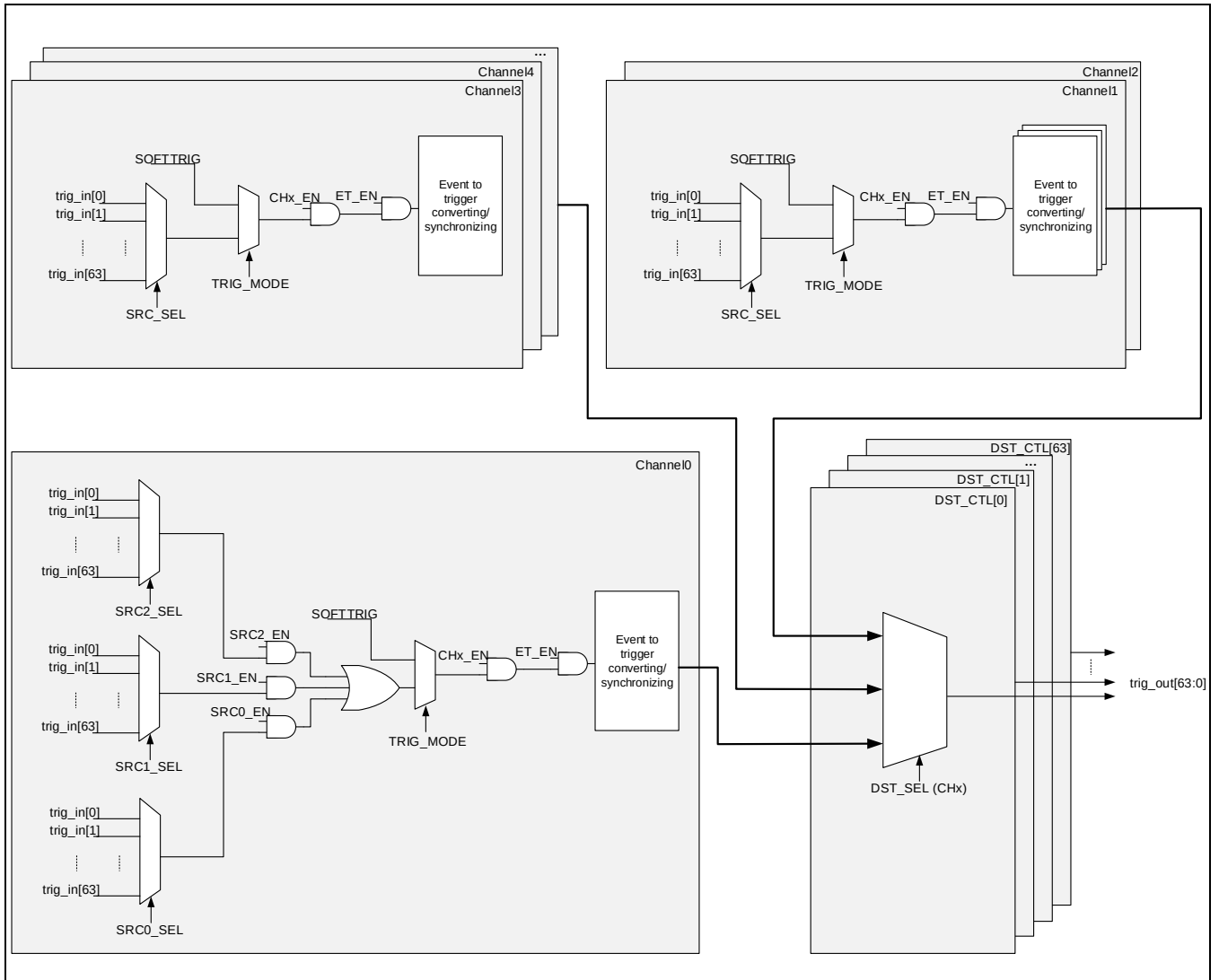
Figure 8-1 ET模块框图
