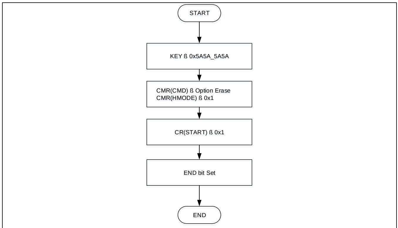
Figure 6-11 Option Cells Erase
