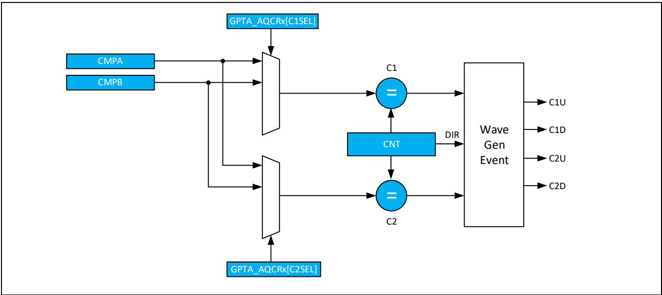
Figure 12-15 C1 and C2 selection control
