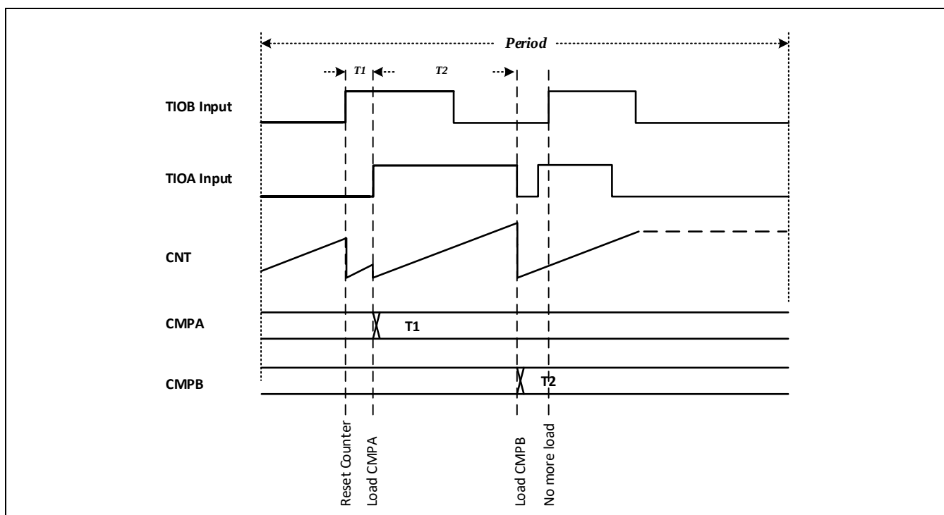
Figure 12-24 测量TIOA和TIOB相位差
