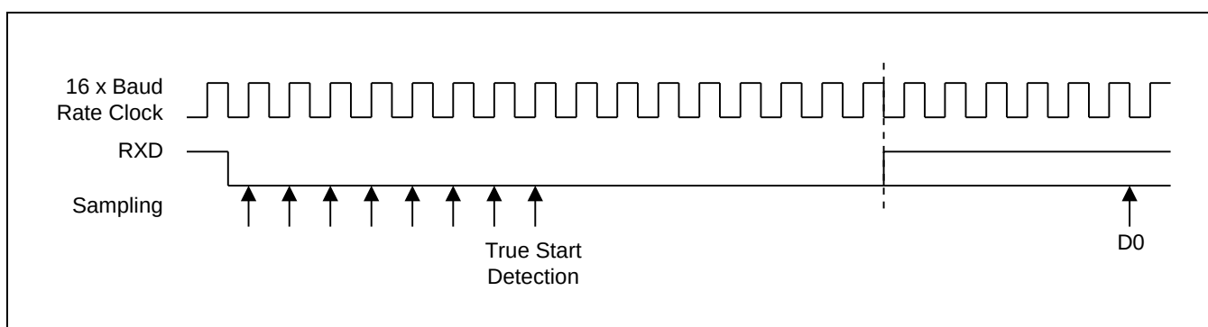
Figure 17-3 异步模式, 起始位检测
