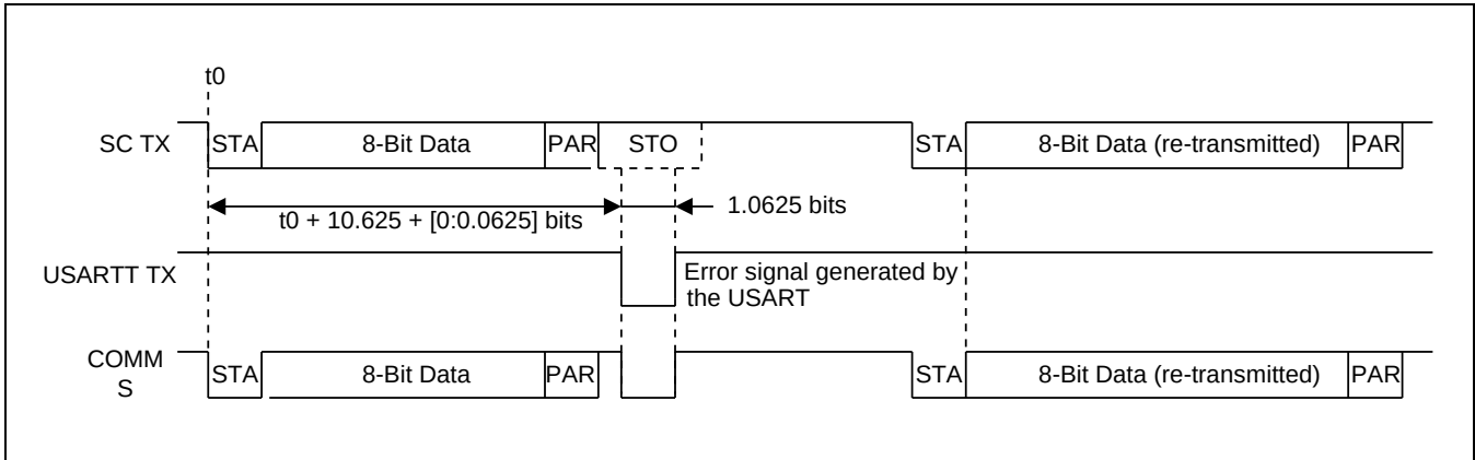
Figure 17-9 接收端的错误检测
