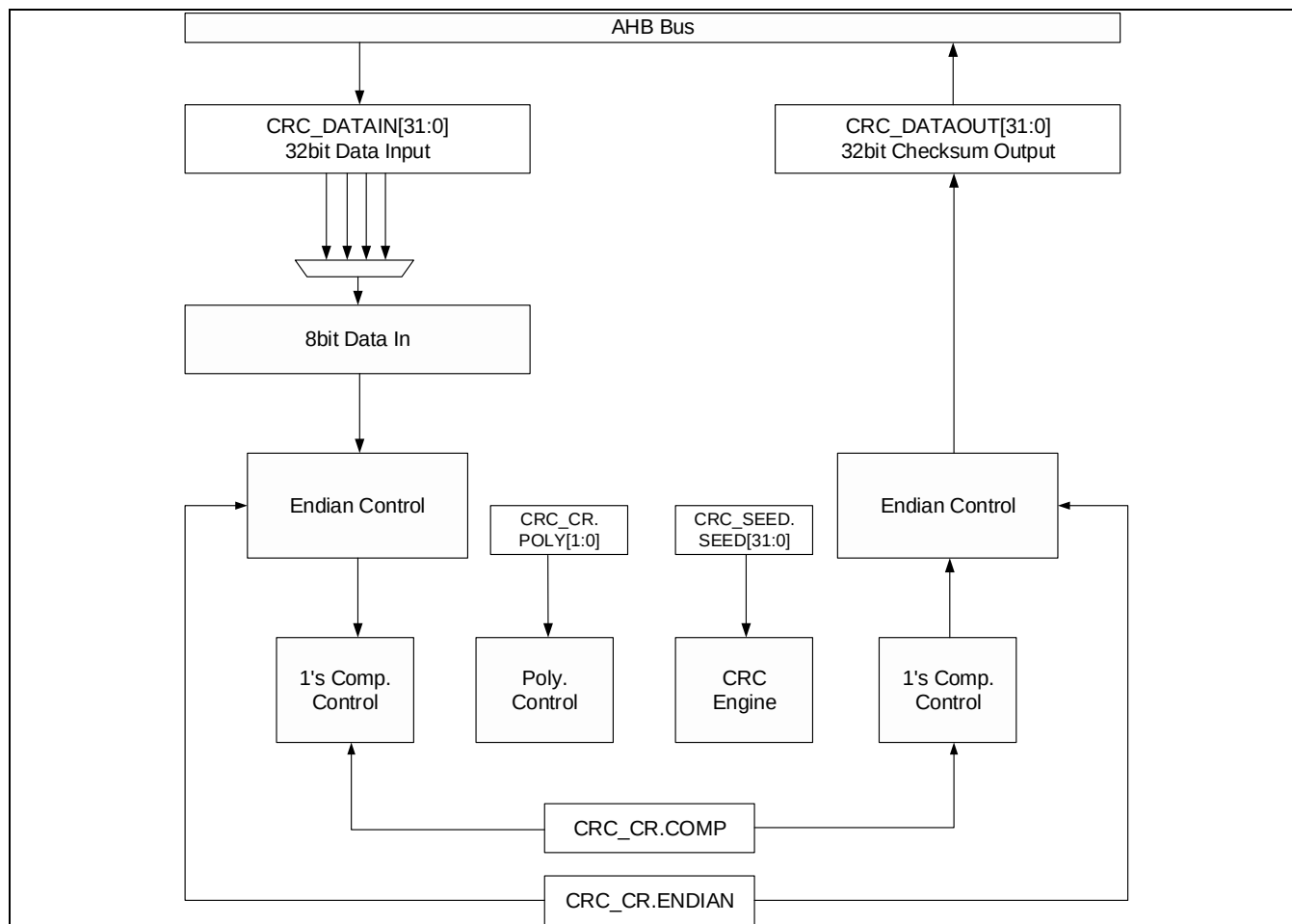
Figure 4-1 CRC模块框图
