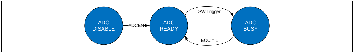
Figure 9-3 ADC状态机
