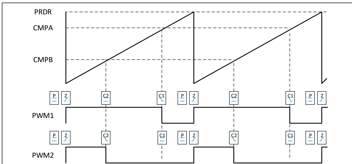
Figure 12-19 递增单沿，非对称波形输出
