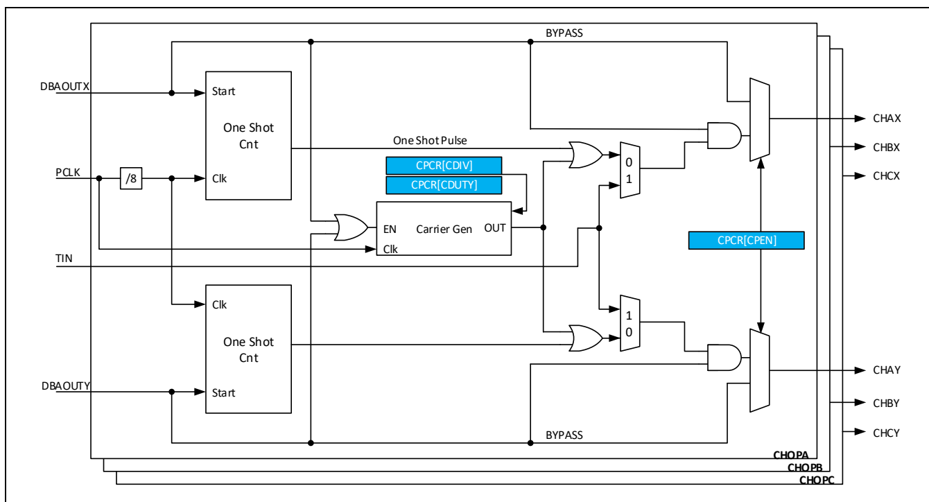
Figure 13-31 斩波使能模块
