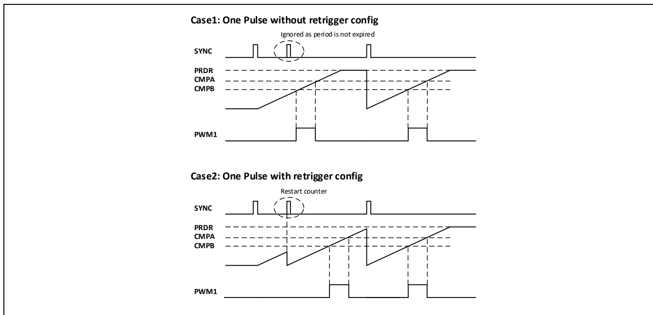
Figure 12-26 单次触发
