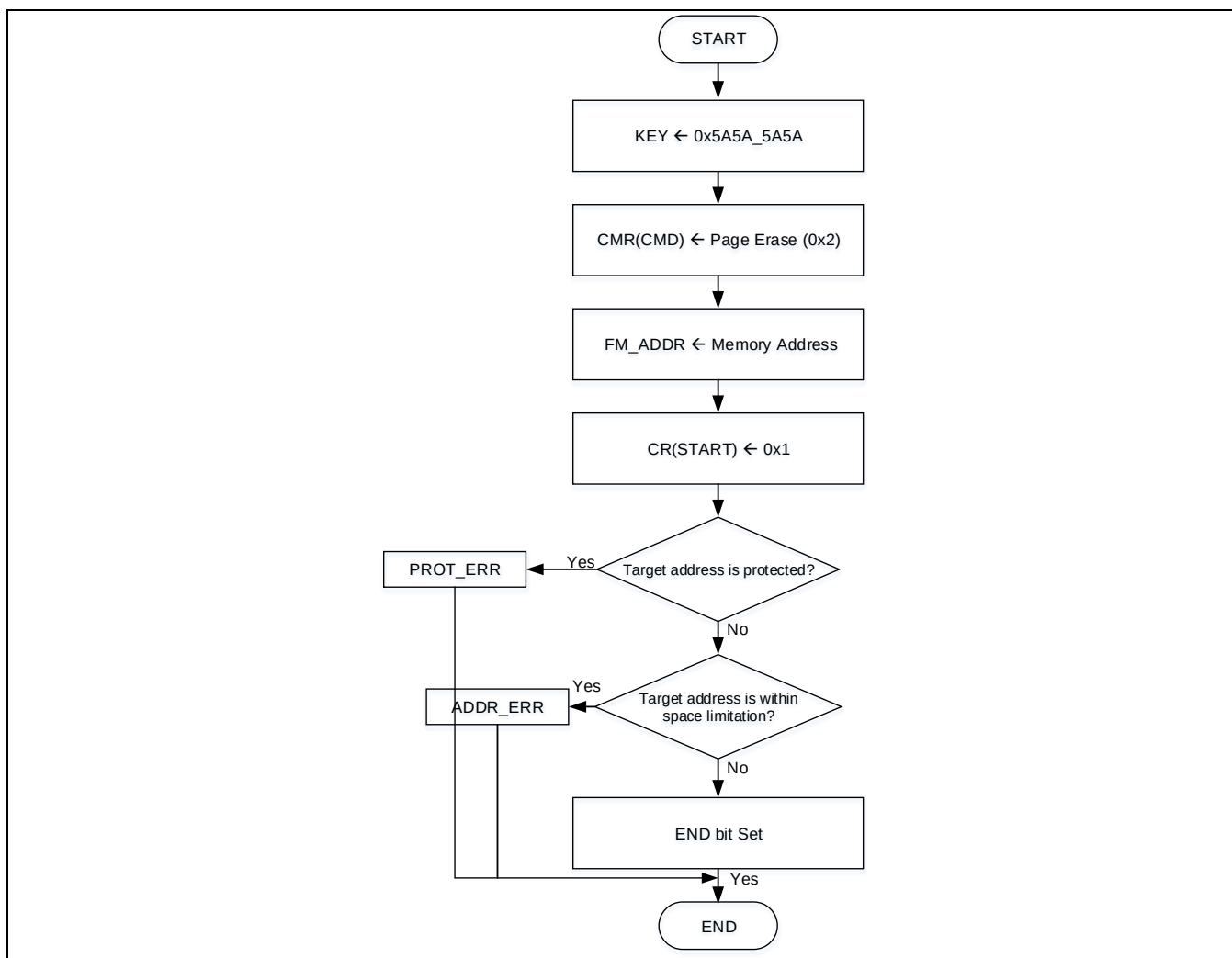
Figure 6-8 Page Erase
