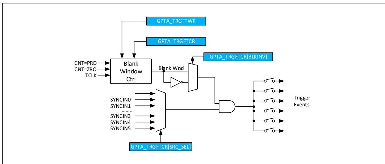
Figure 12-28 滤波器框图
