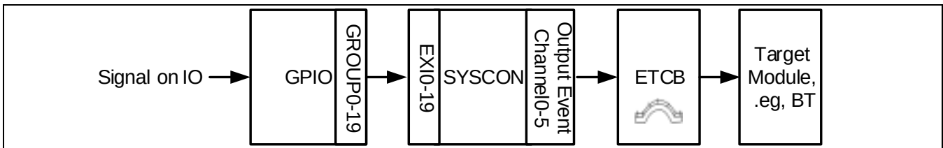
Figure 7-12 Signal Flow
