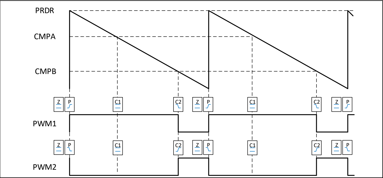
Figure 12-21 递减单沿，非对称波形输出
