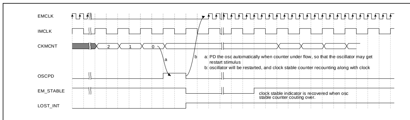
Figure 7-6 EMOSC 失效监测
