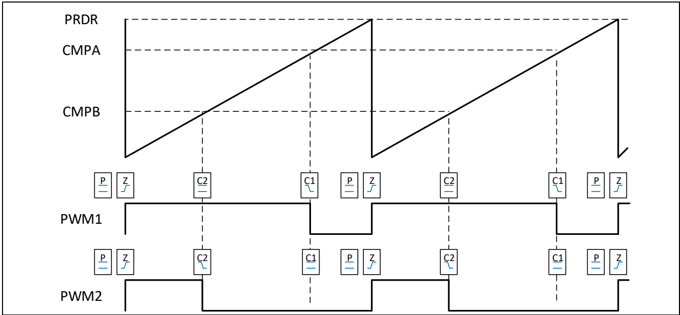
Figure 13-16 递增单沿，非对称波形输出
