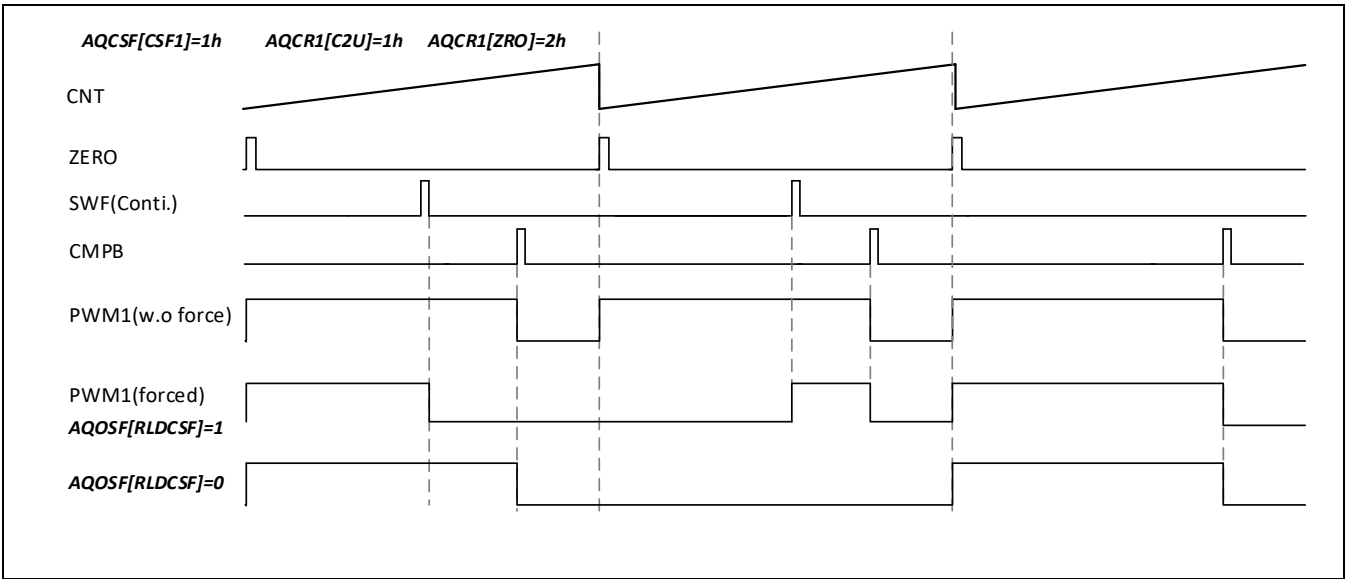
Figure 13-21 持续性软件强制输出
