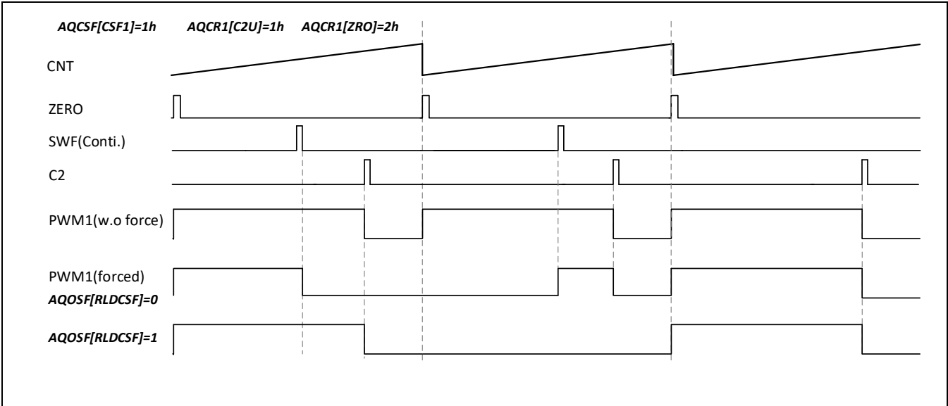
Figure 12-17 持续性软件强制输出
