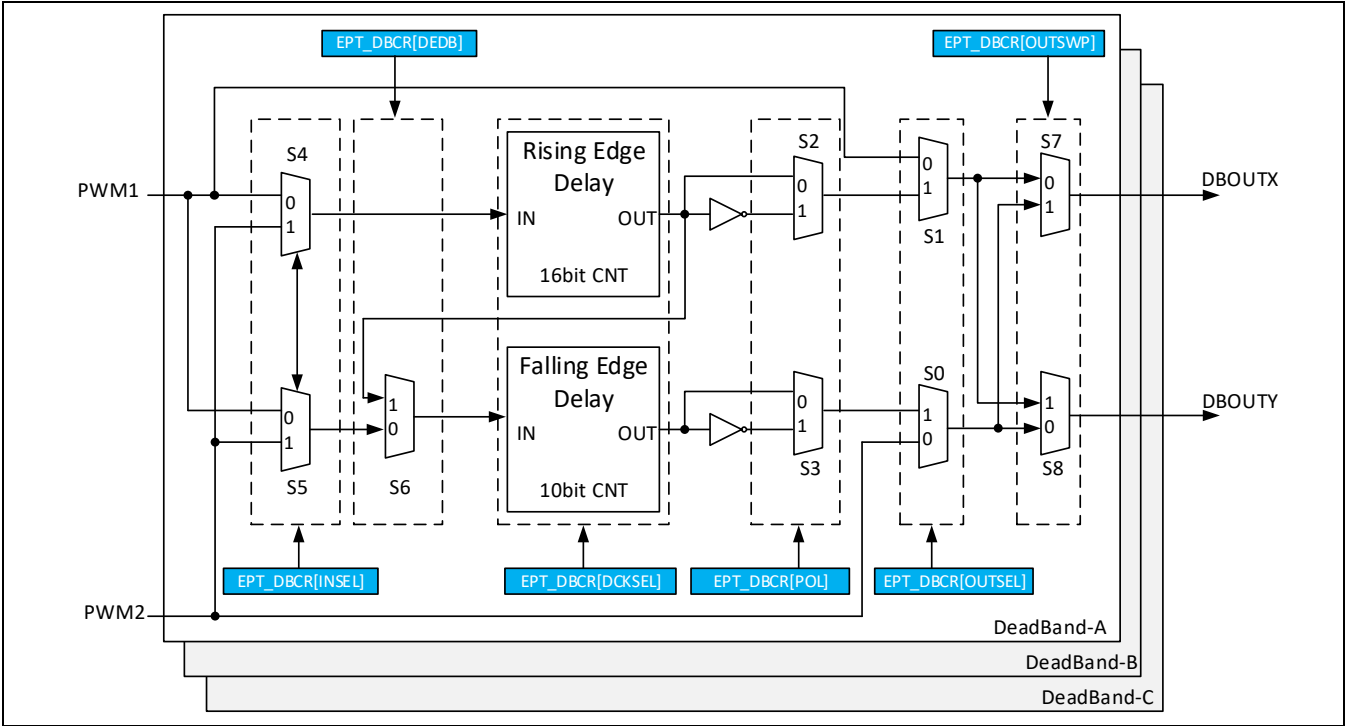
Figure 13-26 死区控制模块
