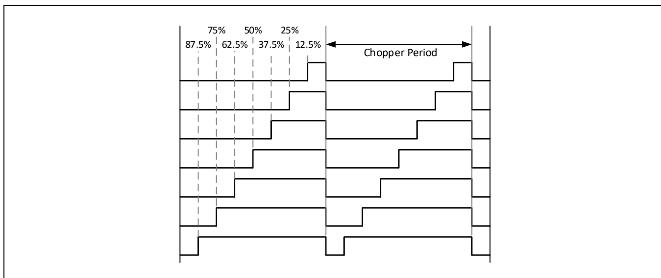
Figure 13-34 载波的占空比
