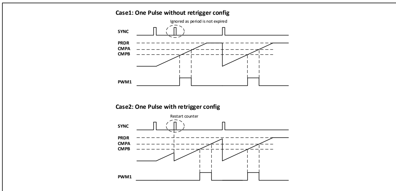
Figure 13-40 单次触发
