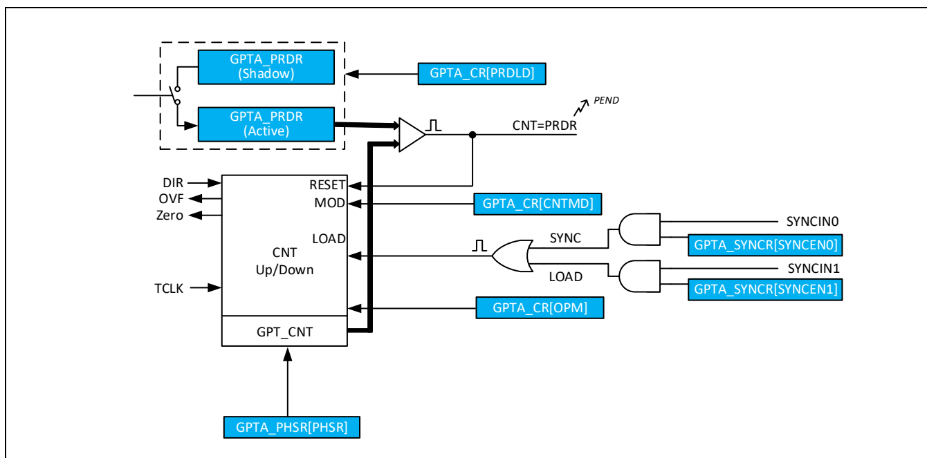
Figure 12-5 计数器时基模块
