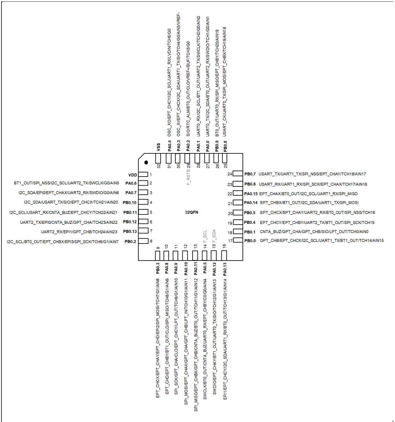
Figure 2-2 管脚定义图(32QFN)
