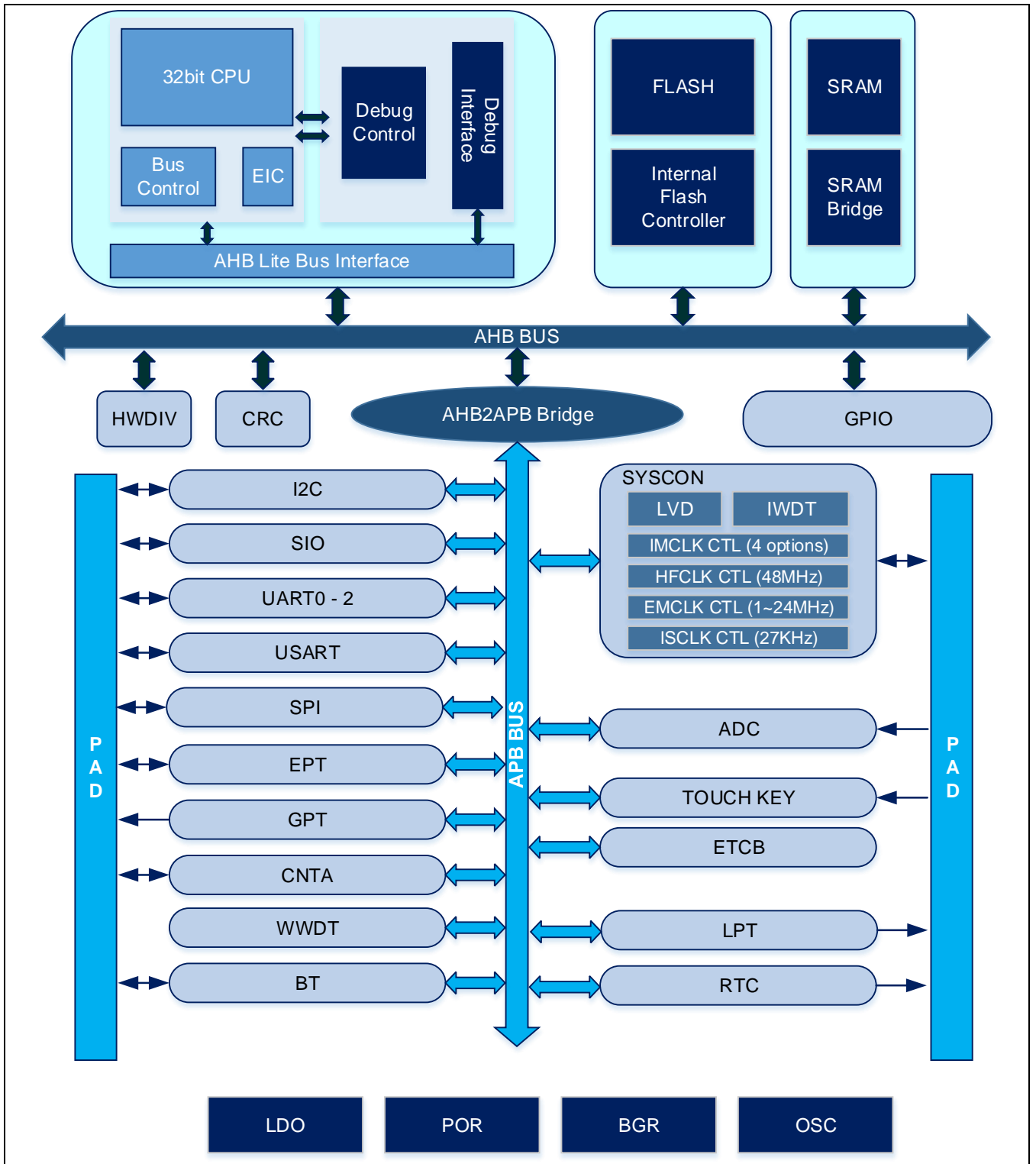
Figure 1-1 APT32S2028模块框图
