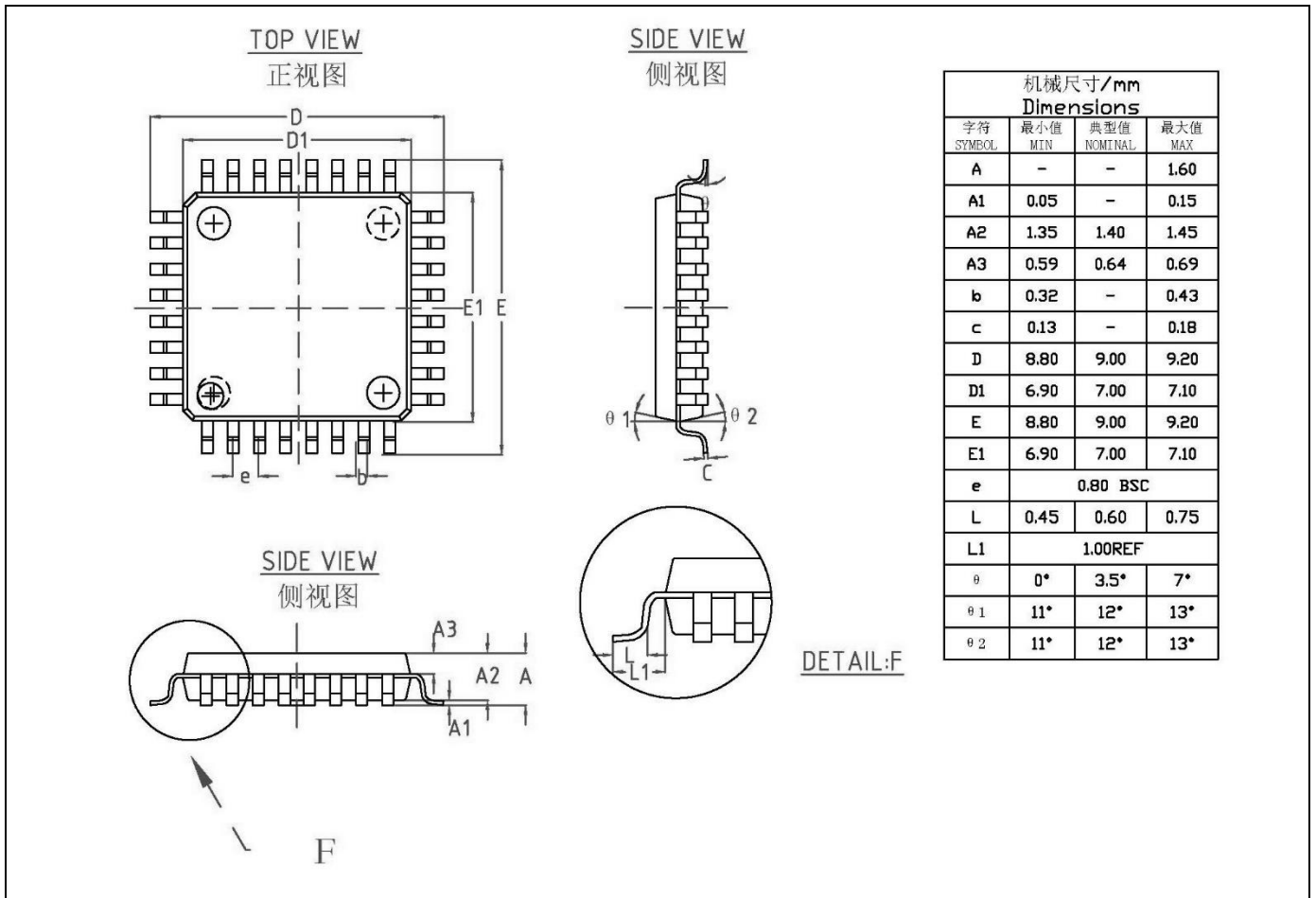
Figure 4-1 32-LQFP封装尺寸
