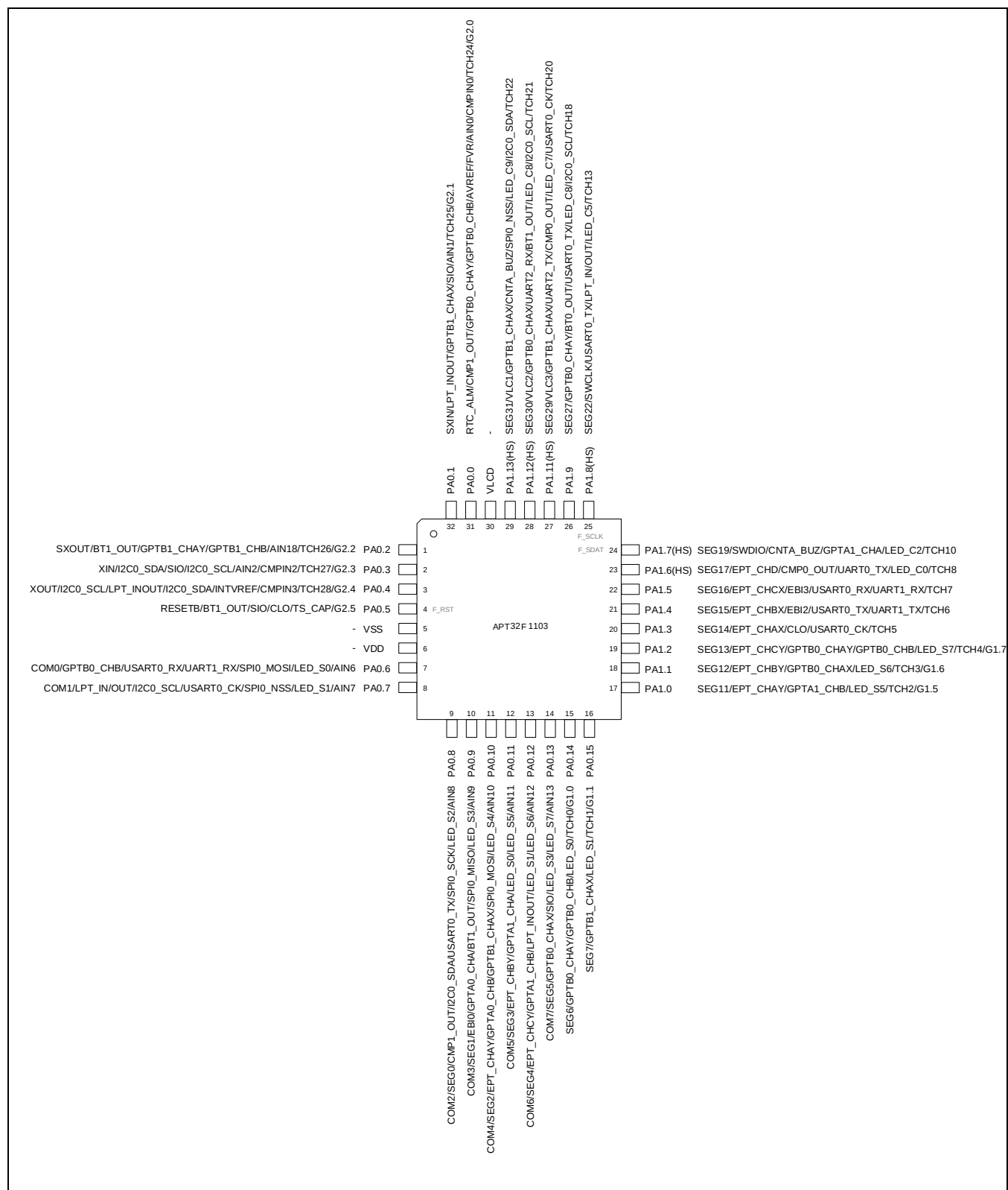
Figure 2-3 管脚定义图(32 LQFP/QFN)
