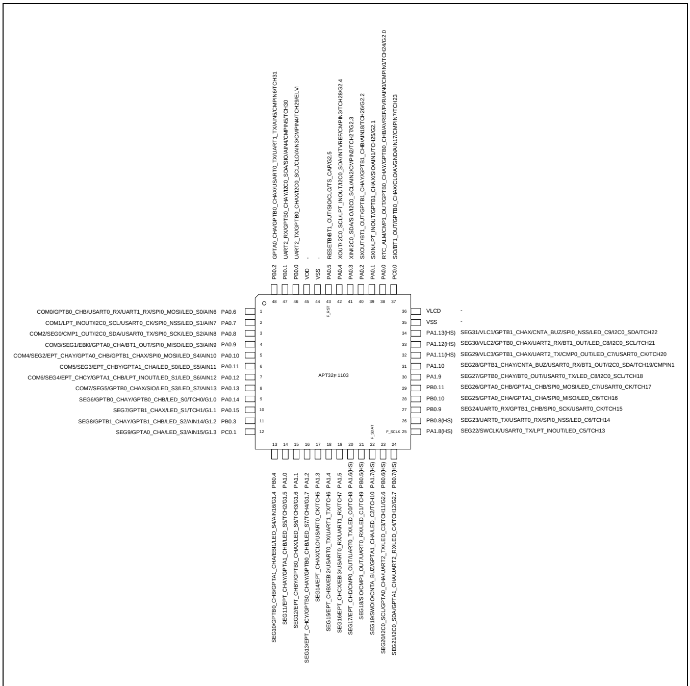
Figure 2-1 管脚定义图(48 LQFP/QFN)
