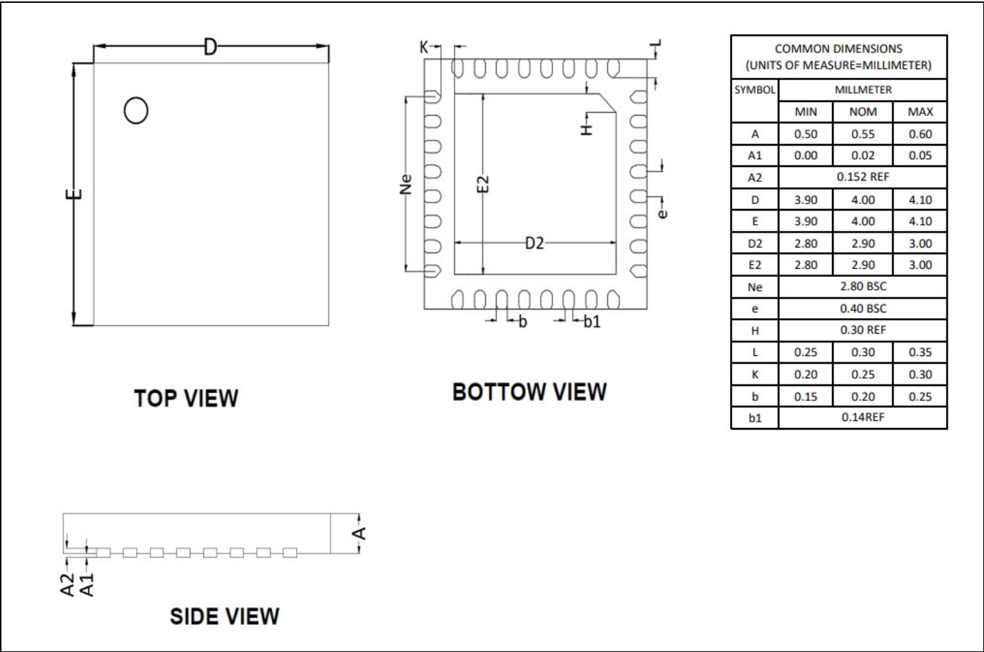
Figure 4-5 32-QFN (4x4-P0.4mm)封装尺寸
