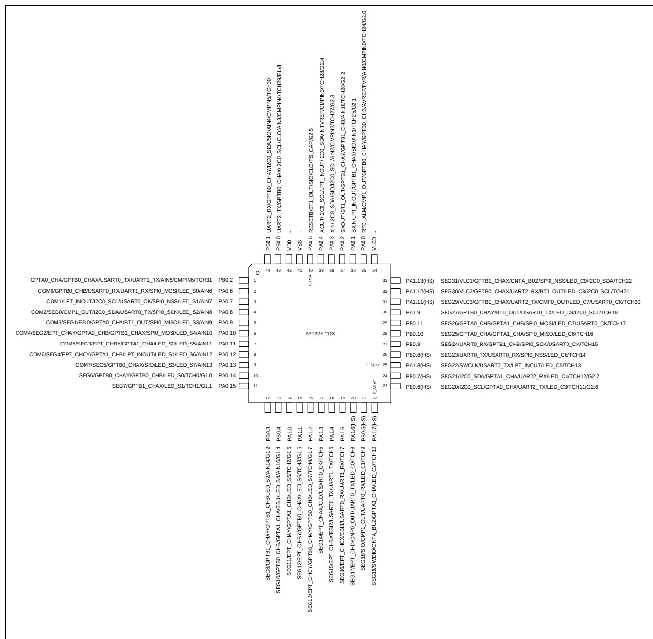
Figure 2-2 管脚定义图(44 LQFP)
