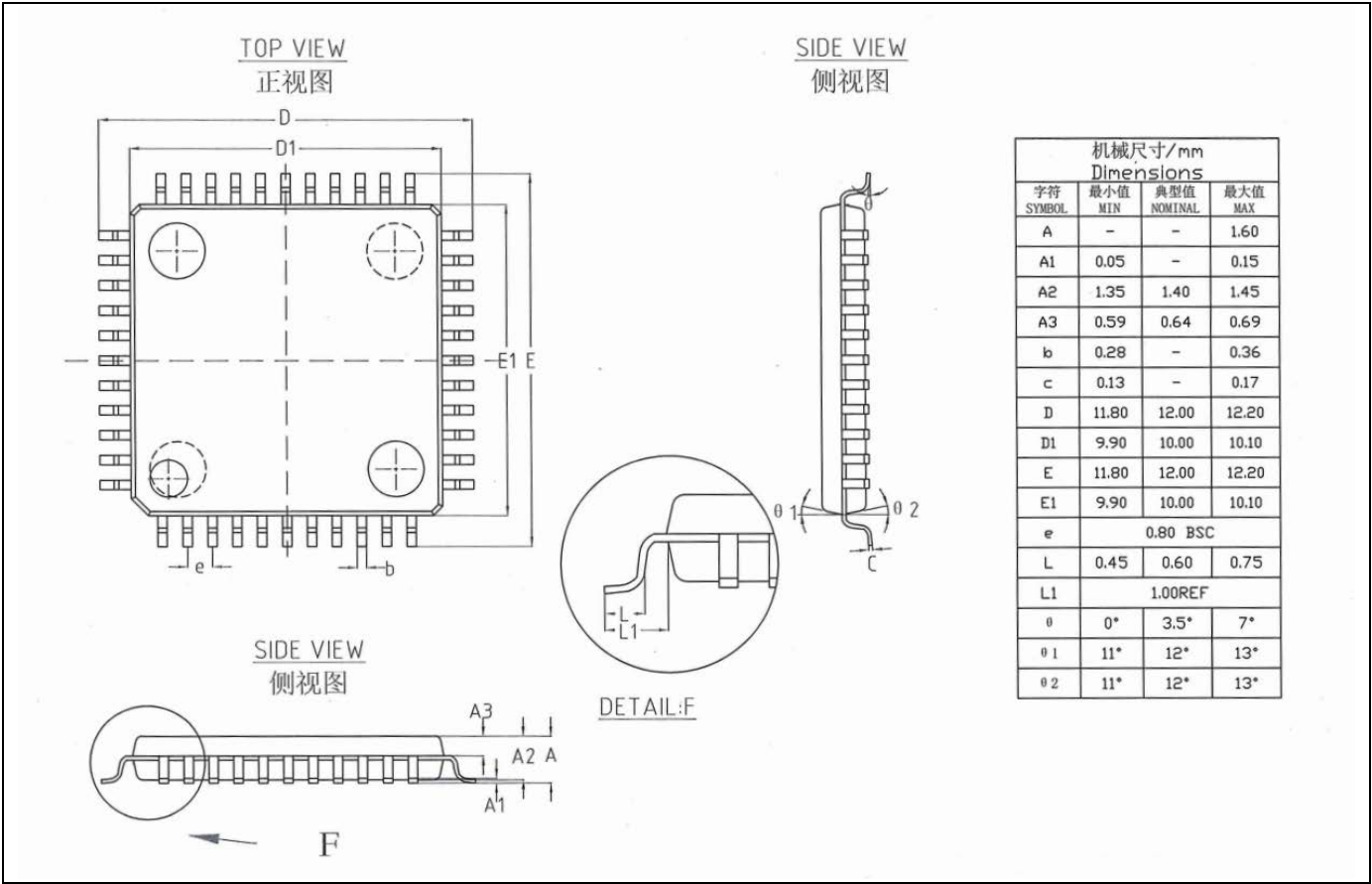
Figure 4-3 44-LQFP (10x10-P0.8mm) 封装尺寸
