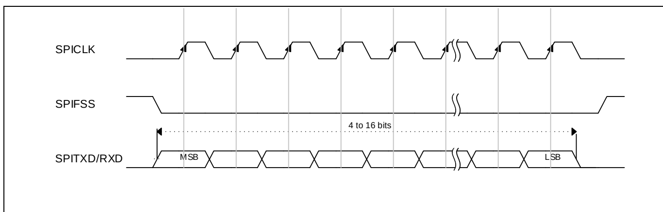
Figure 14-5 Motorola SPI 帧格式 (单帧传输) SPO = 0, SPH = 0
