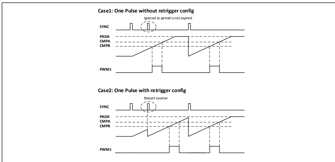
Figure 10-15 单次触发
