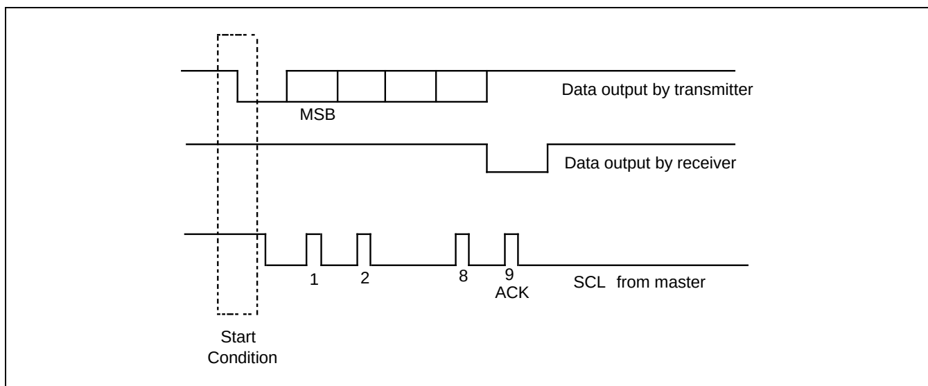
Figure 13-5 应答
