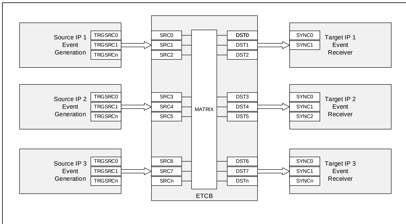
Figure 7-2 IP间通过ETCB事件同步
