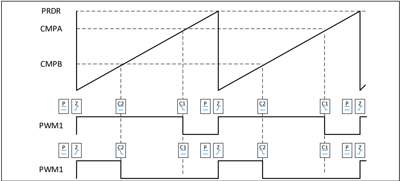
Figure 10-11 递增单沿，非对称波形输出
