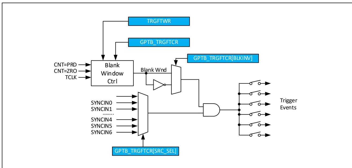
Figure 11-31 滤波器框图
