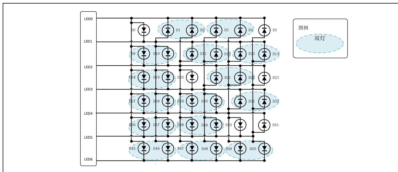
Figure 17-9 6*6点阵驱动
