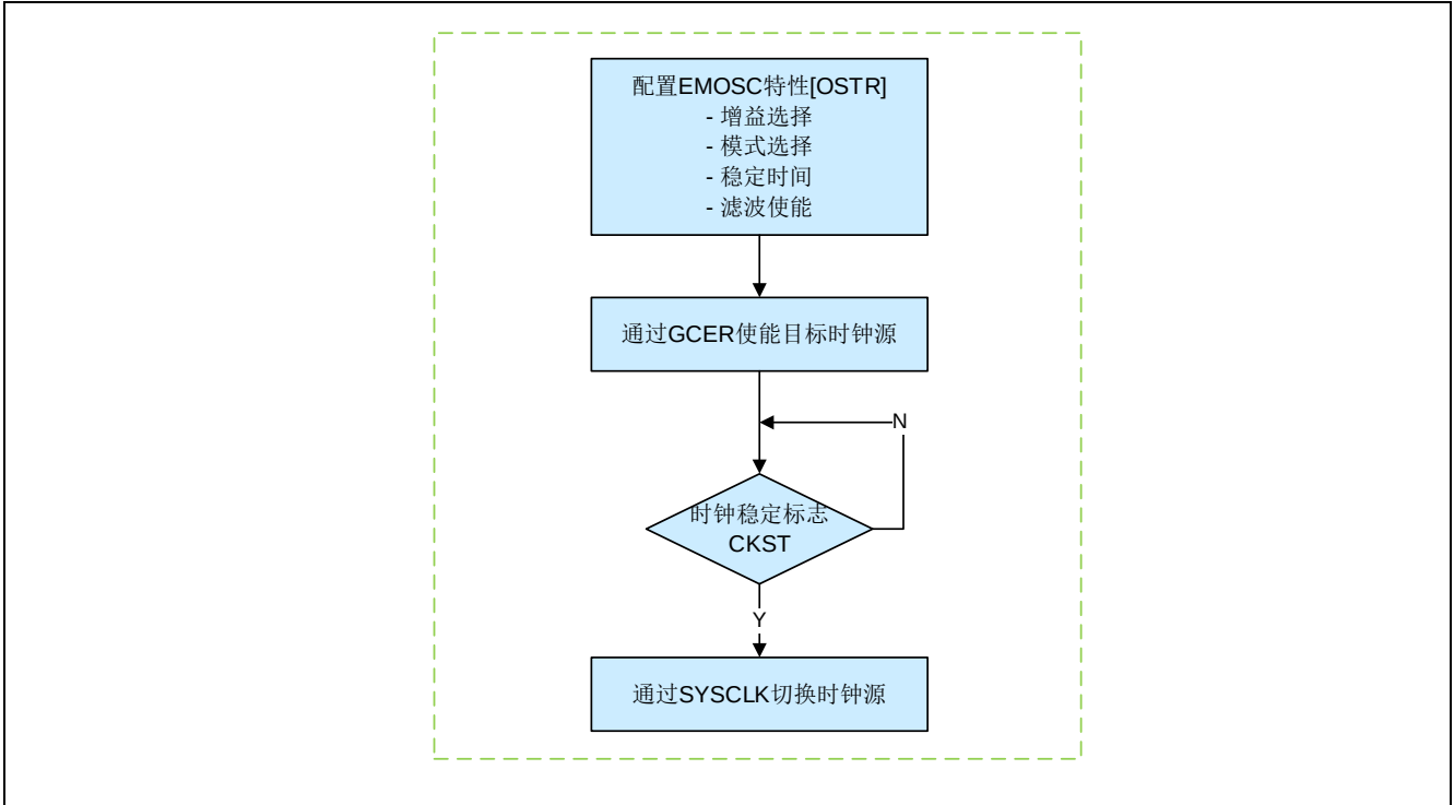
Figure 5-5 配置外部时钟源
