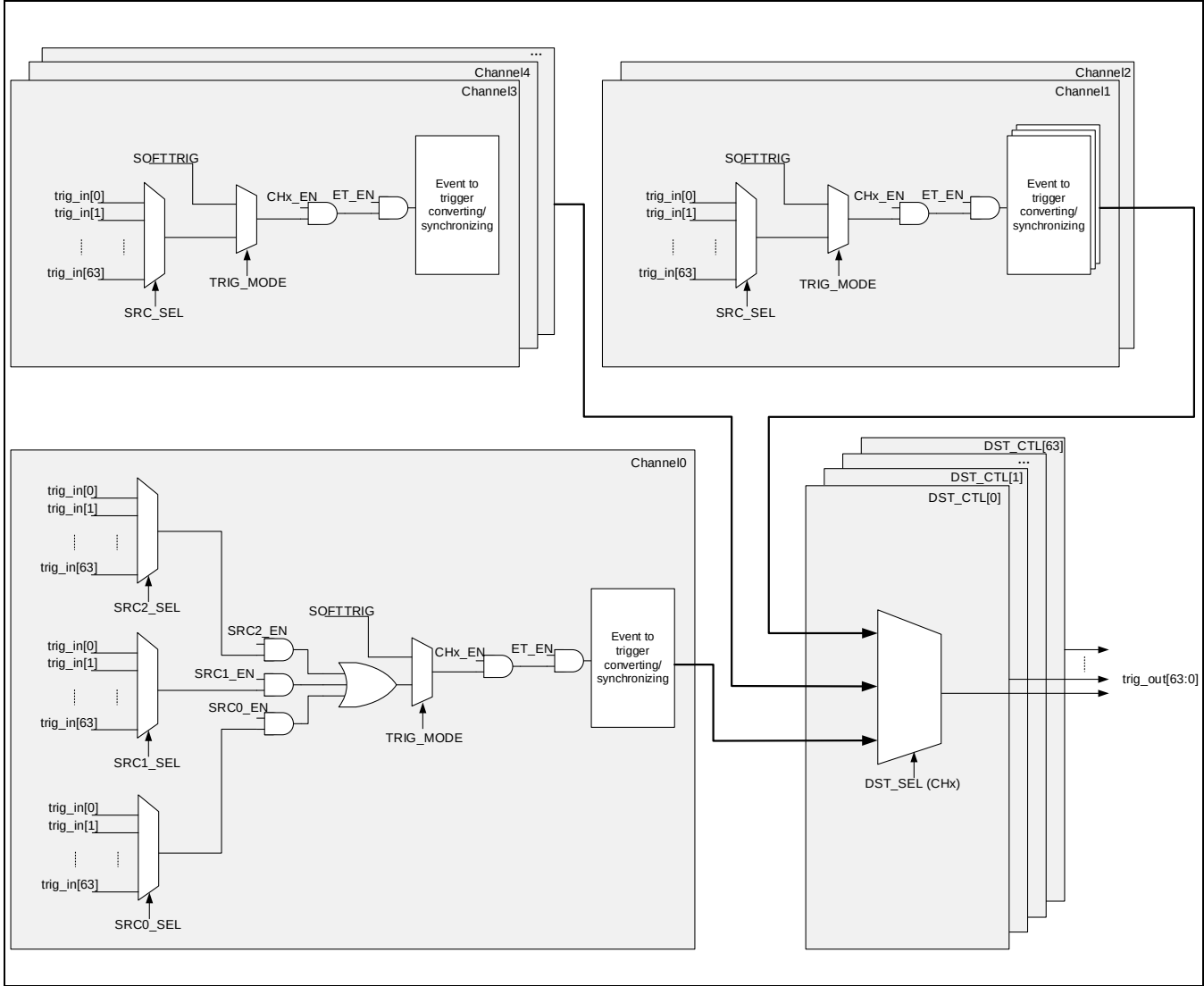
Figure 7-1 ETCB模块框图
