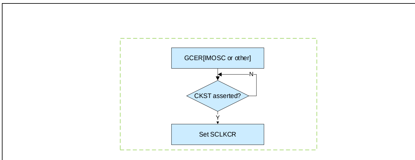
Figure 5-4 配置内部时钟源
