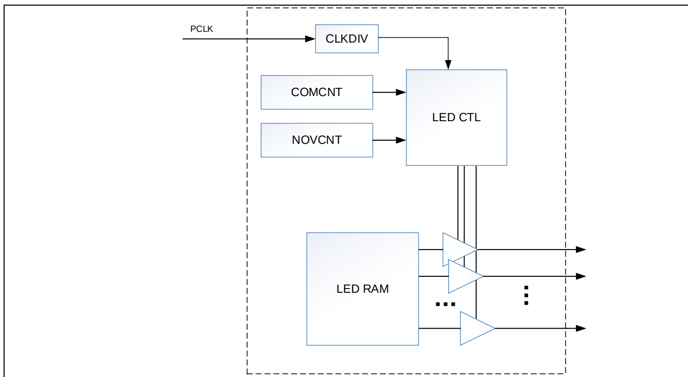
Figure 17-1 LED 扫描模块功能图
