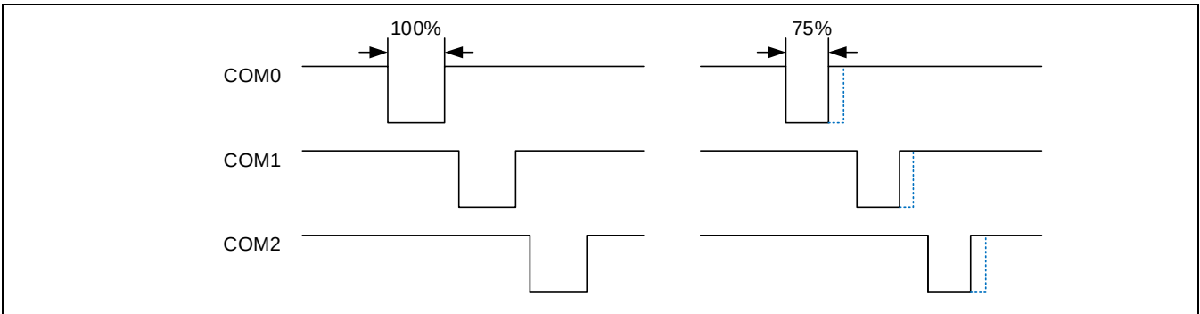
Figure 17-4 LED 显示亮度调节
