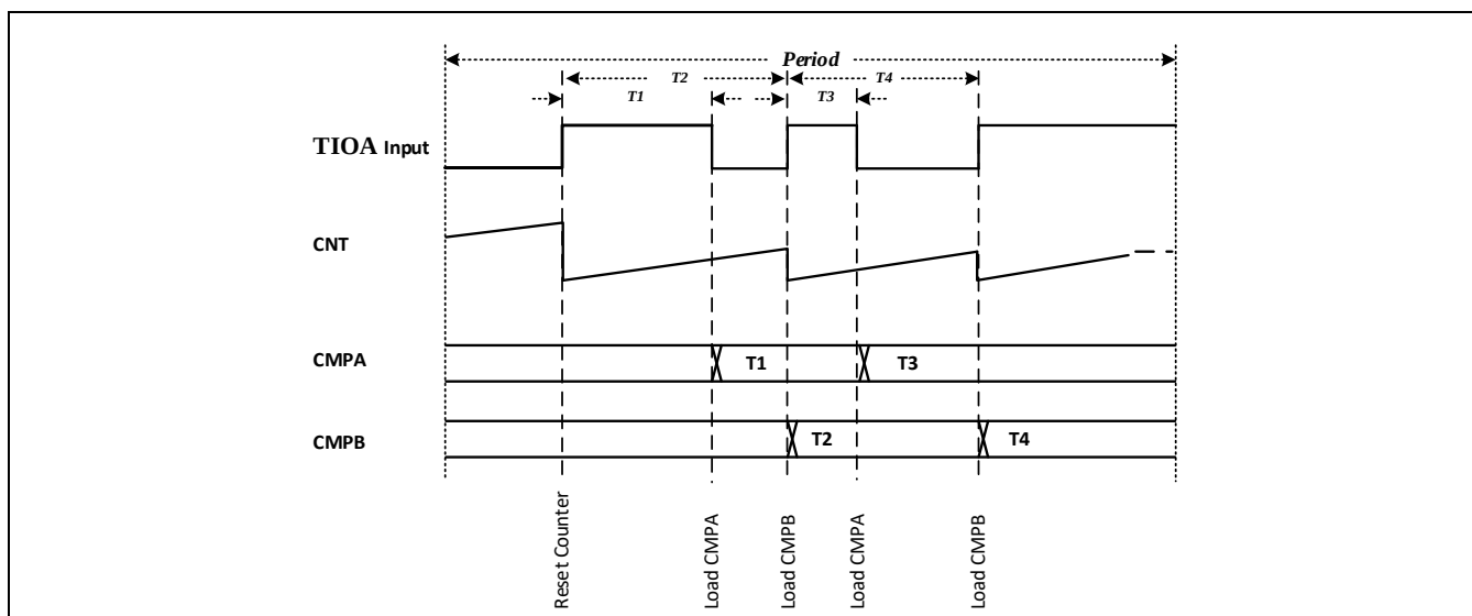
Figure 11-28 CHA的脉冲宽度和周期
