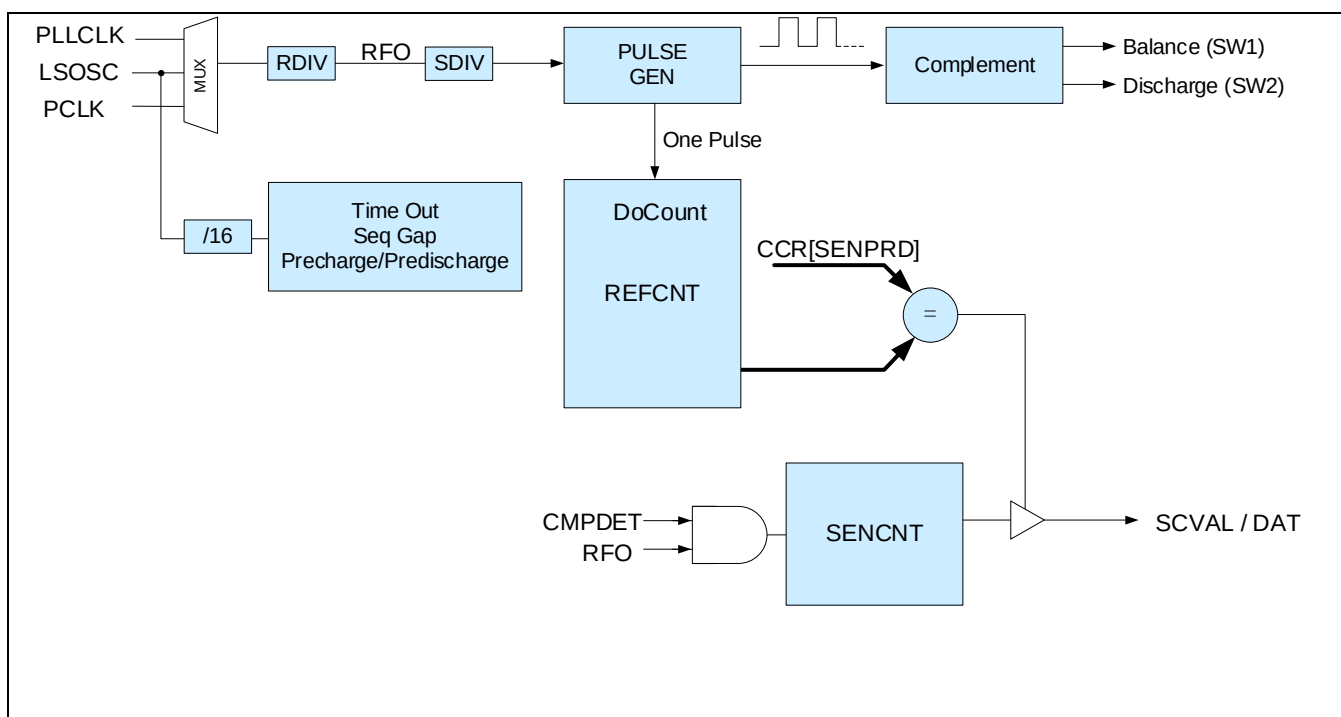
Figure 18-2 Touch Sensor数字框图
