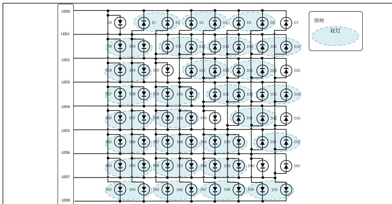
Figure 17-6 8*8点阵驱动
