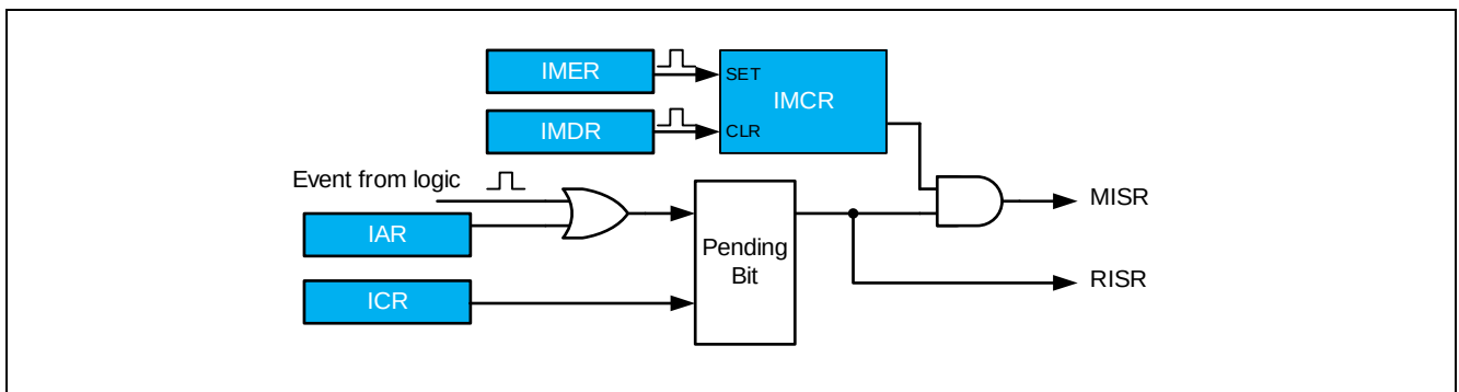
Figure 5-12 SYSCON 通用中断的控制逻辑
