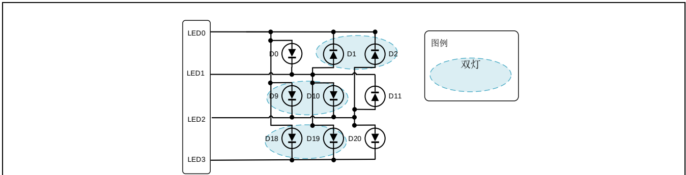
Figure 17-13 3*3点阵驱动
