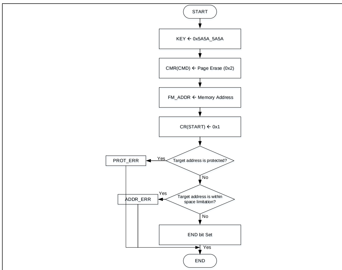
Figure 4-7 Page Erase
