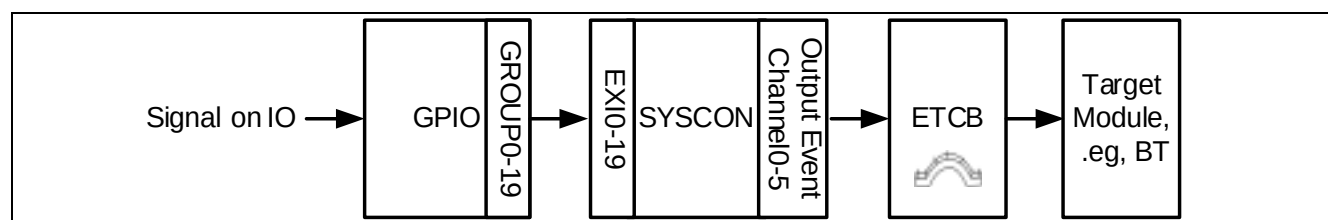
Figure 5-13 Signal Flow
