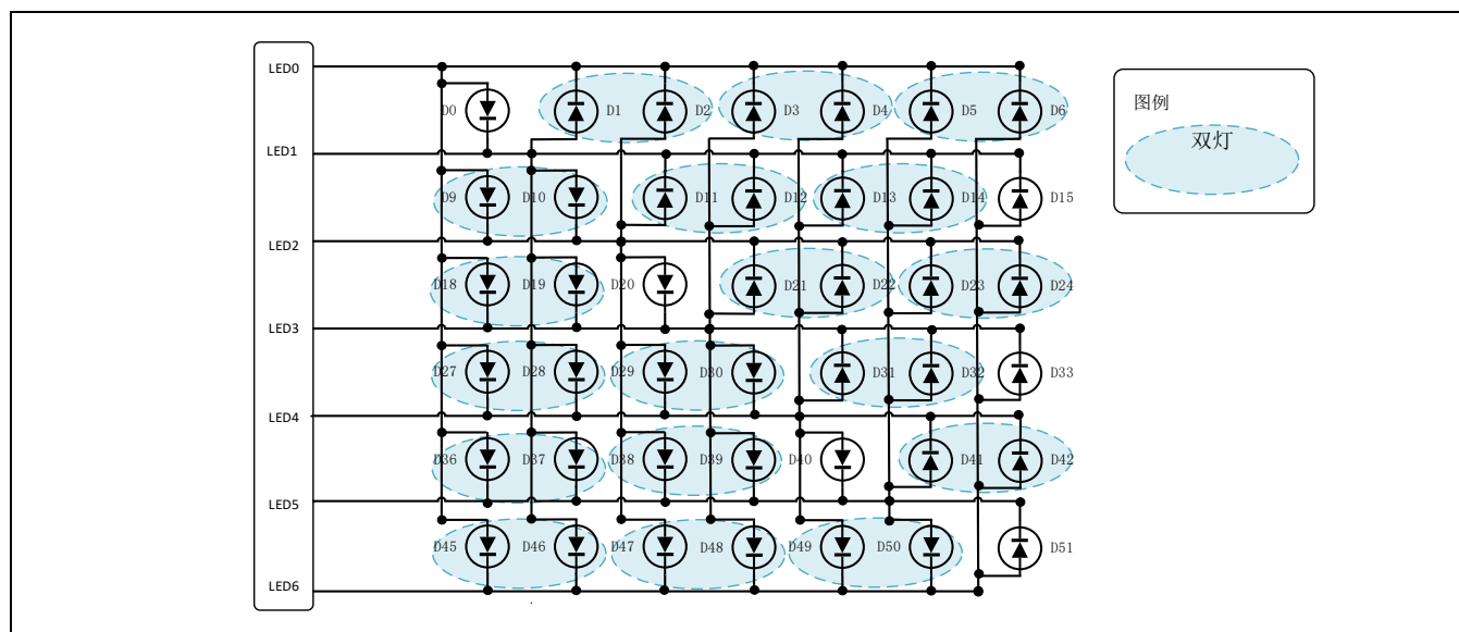
Figure 17-8 6*7点阵驱动
