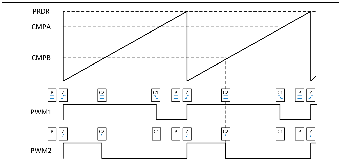
Figure 11-12 递增单沿，非对称波形输出
