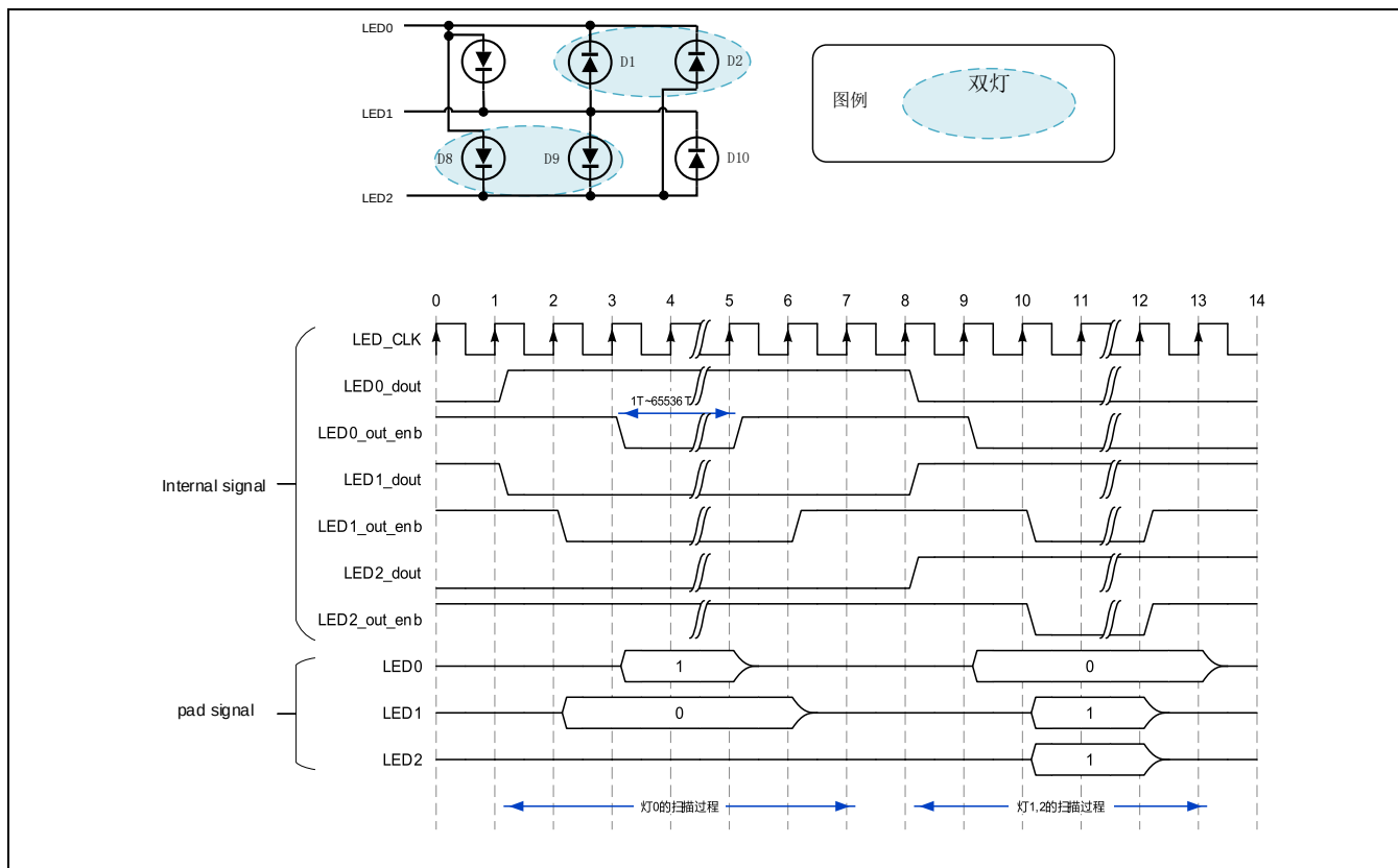
Figure 17-14 点阵驱动数字信号时序图
