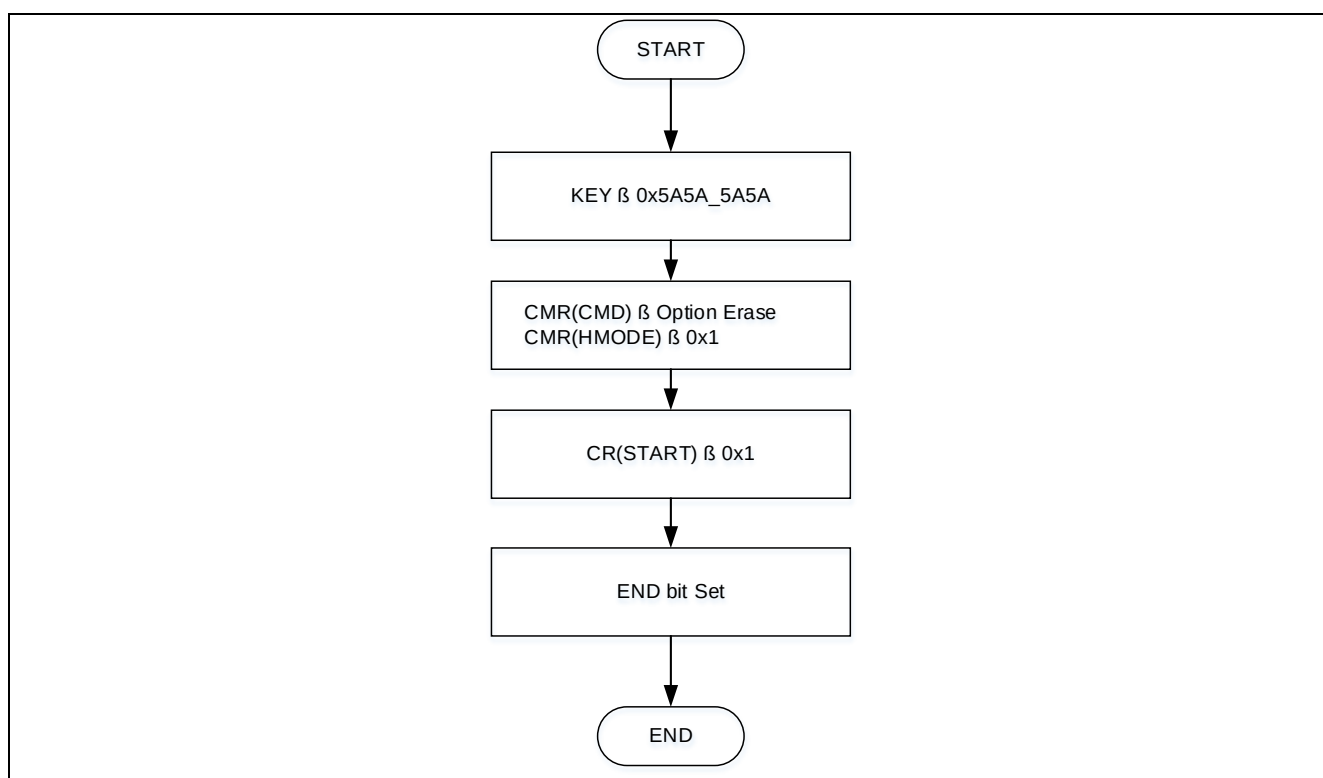
Figure 4-10 Option Cells Erase
