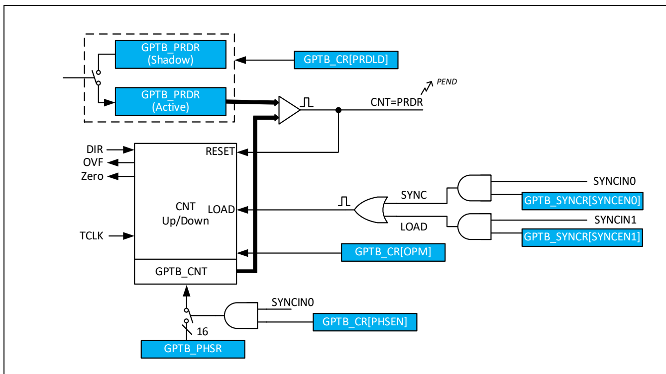
Figure 11-5 计数器时基模块
