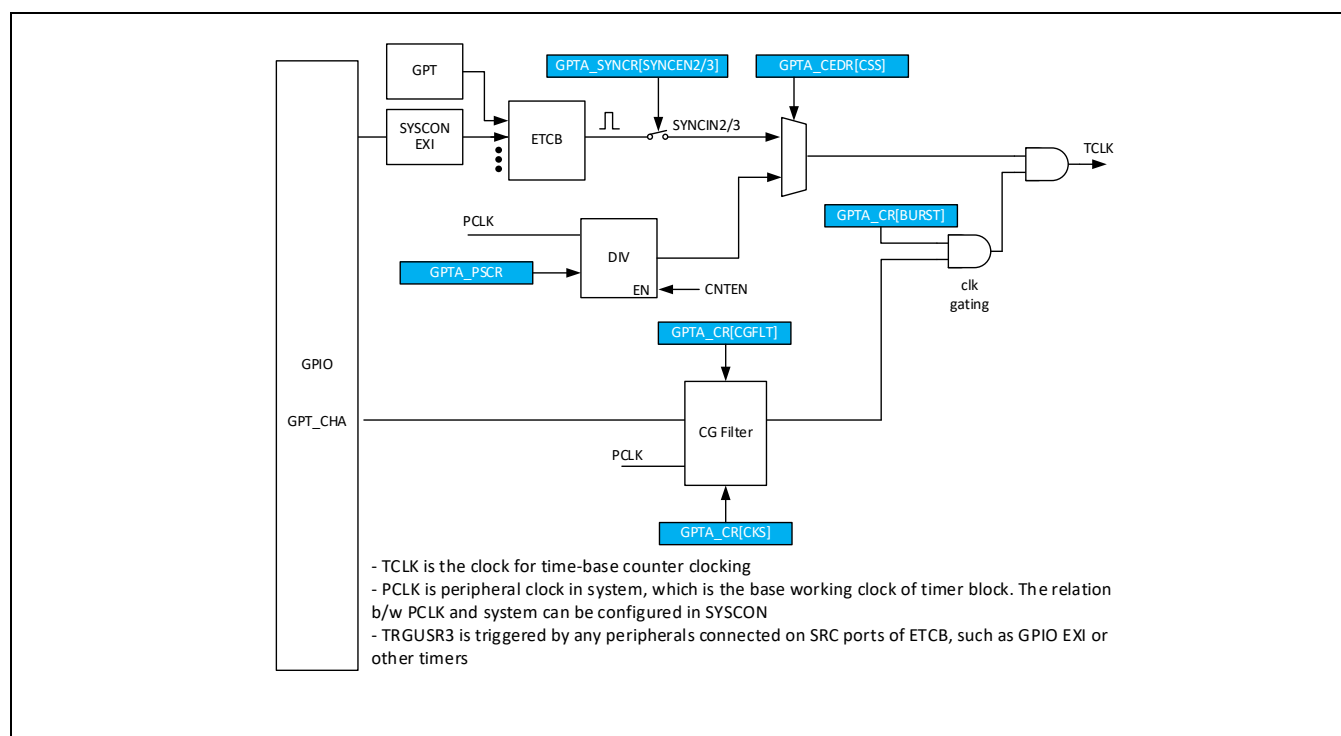
Figure 10-2 时钟控制模块
