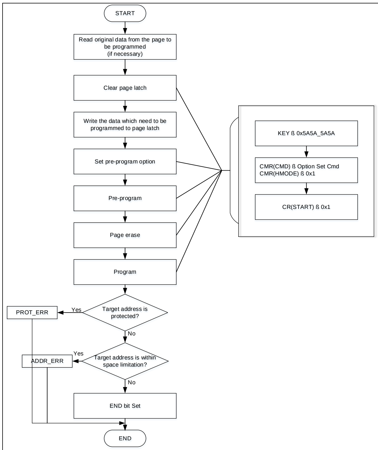
Figure 4-9 Option Cells Write
