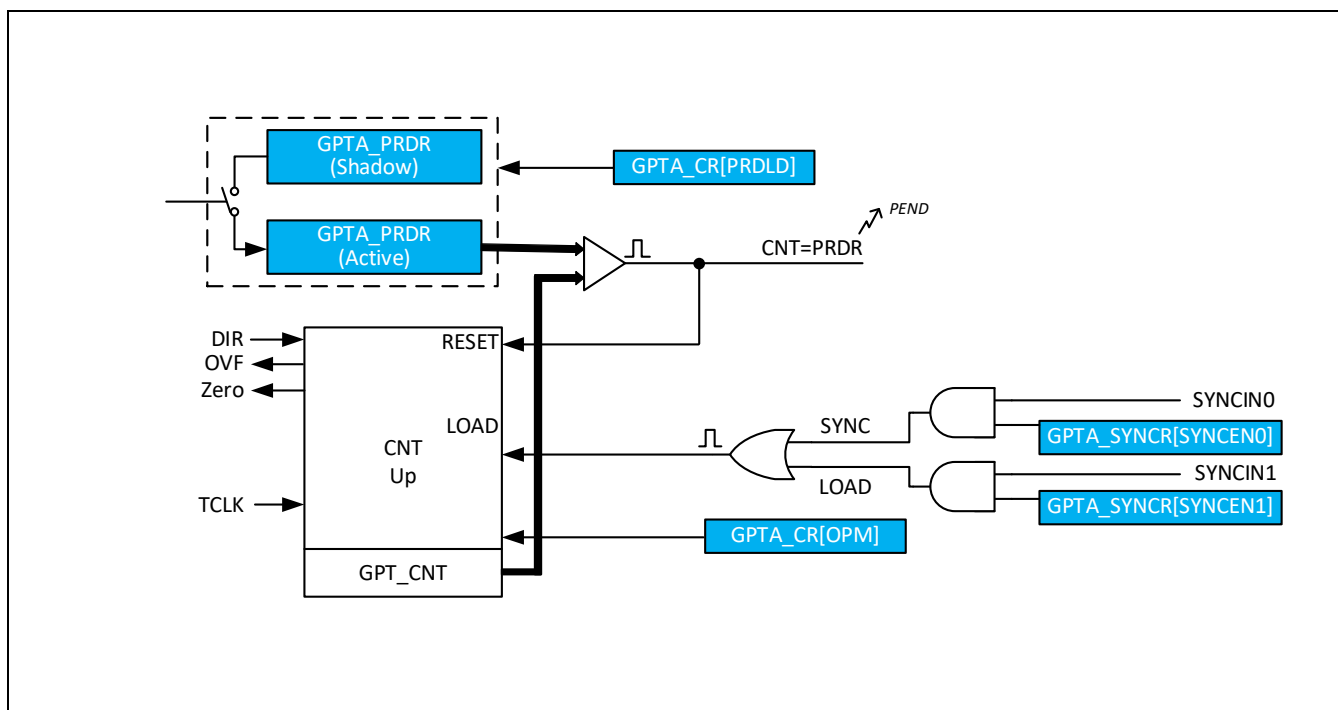
Figure 10-5 计数器时基模块
