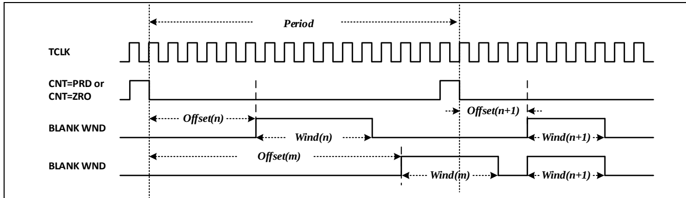
Figure 11-32 滤波器时序
