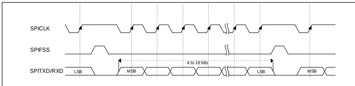
Figure 14-12 Motorola SPI 帧格式(连续传输), SPO = 1 和 SPH = 1
