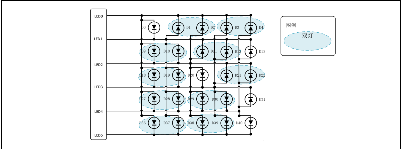
Figure 17-10 5*5点阵驱动
