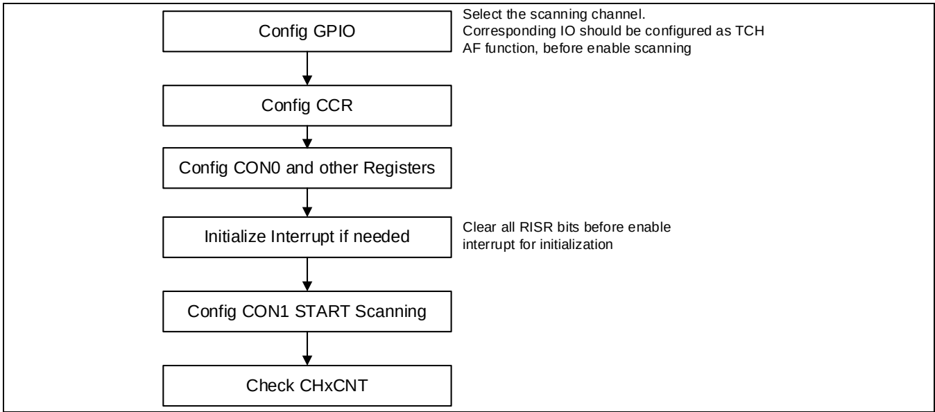
Figure 18-3 软件配置流程
