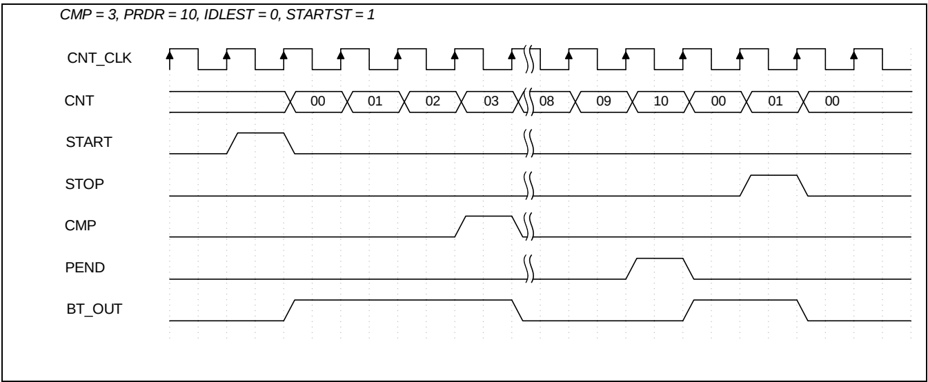
Figure 8-5 BT 输出波形时序图
