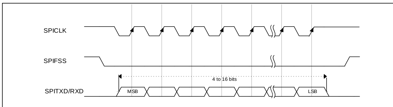
Figure 14-11 Motorola SPI 帧格式(单帧传输), SPO = 1 和 SPH = 1
