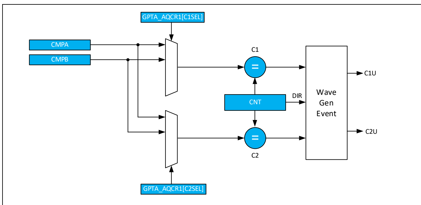
Figure 10-10 C1 and C2 selection control
