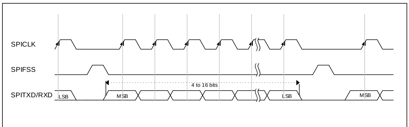
Figure 14-6 Motorola SPI 帧格式 (连续传输) SPO = 0, SPH = 0
