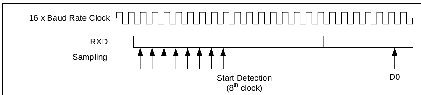
Figure 15-3 起始位检测
