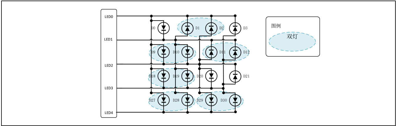
Figure 17-12 4*4点阵驱动
