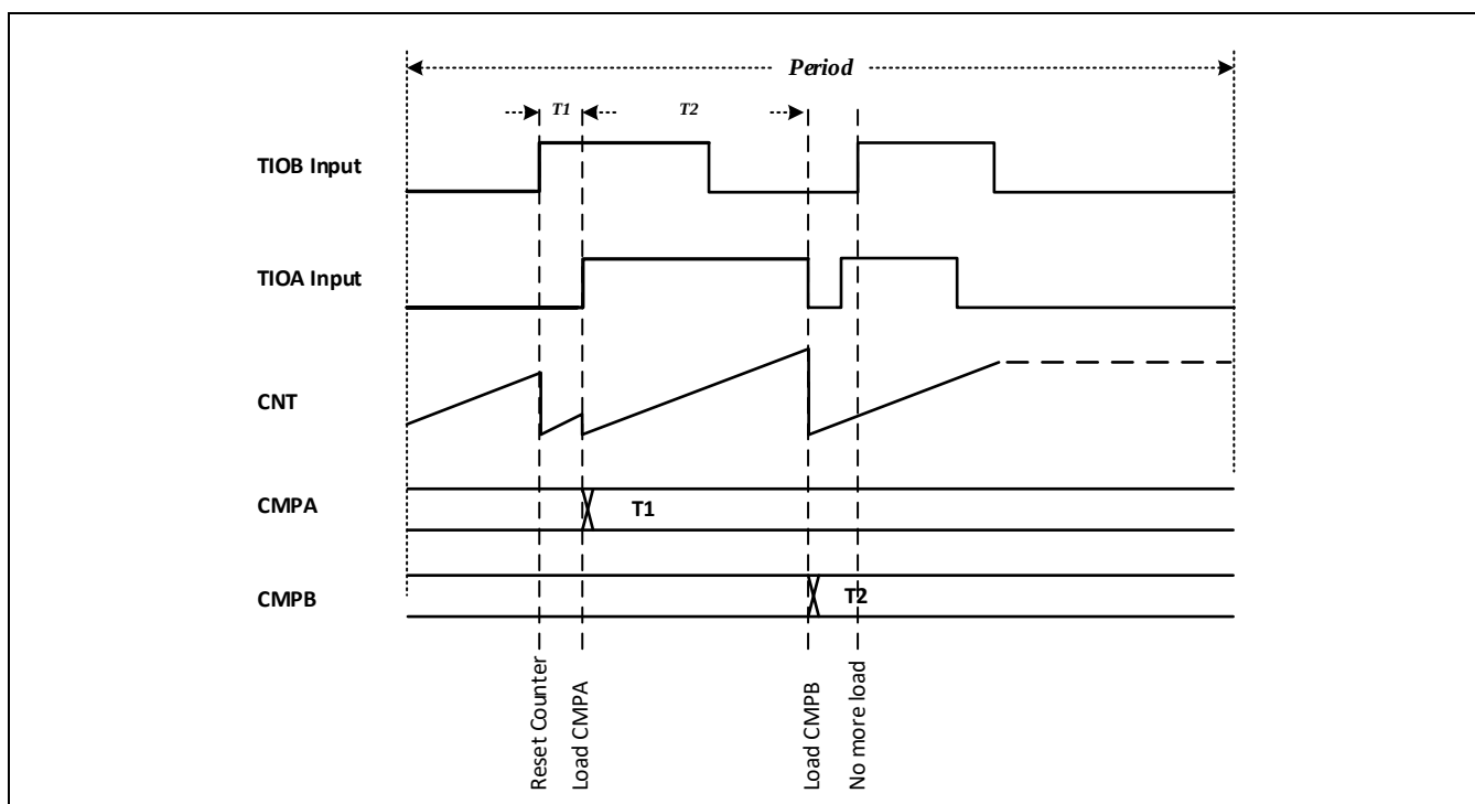
Figure 10-13 测量TIOA和TIOB相位差
