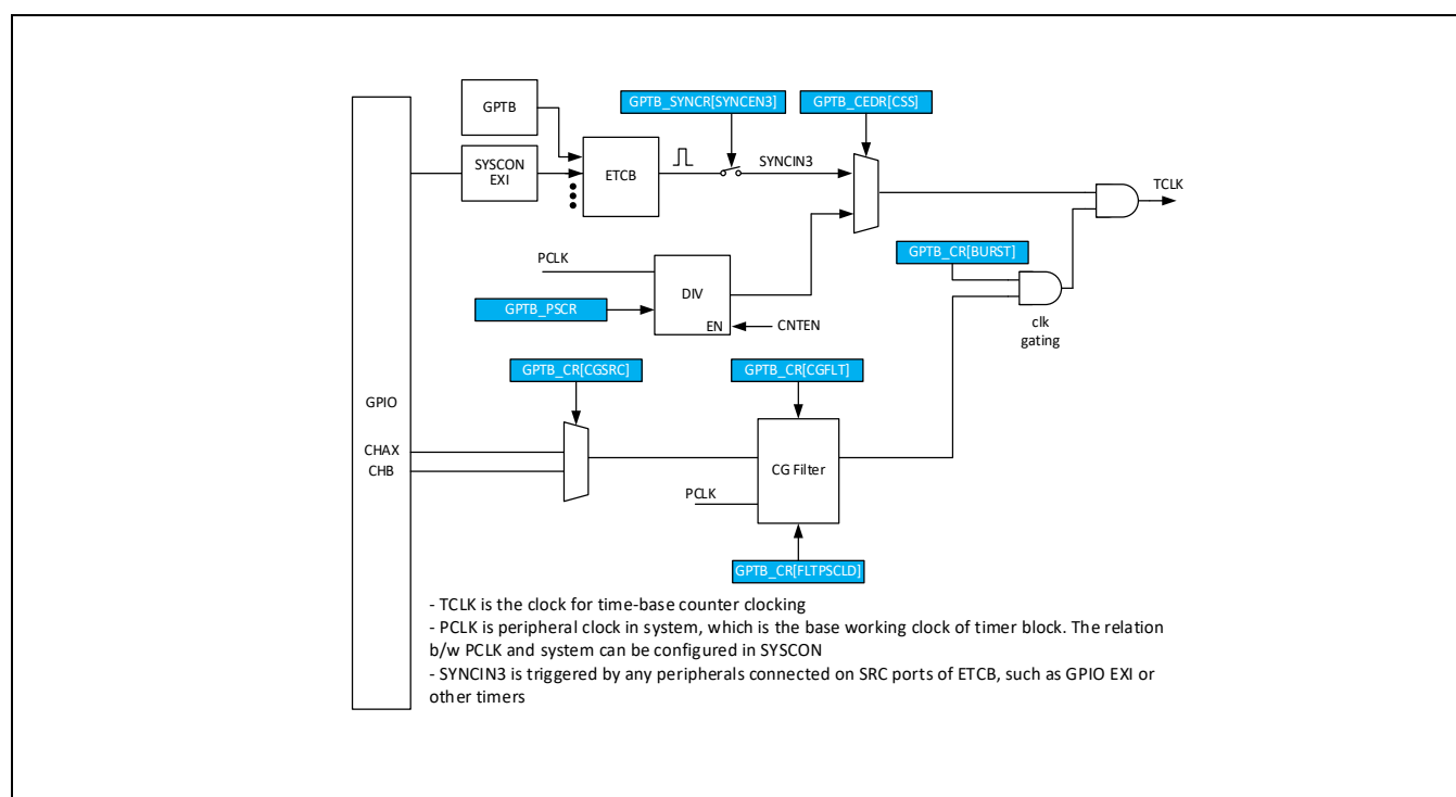
Figure 11-2 时钟控制模块
