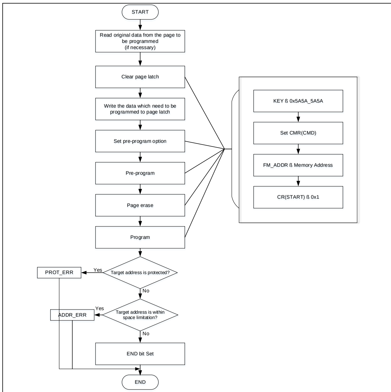
Figure 4-5 Flash Write – Normal Mode
