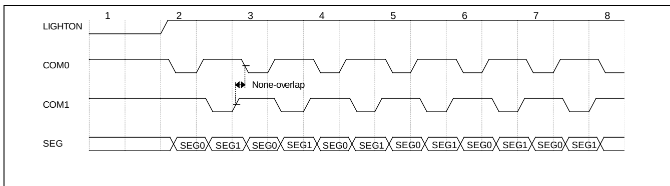
Figure 17-2 LED 扫描显示 (COM_EN = 8'b0000_0011模式)
