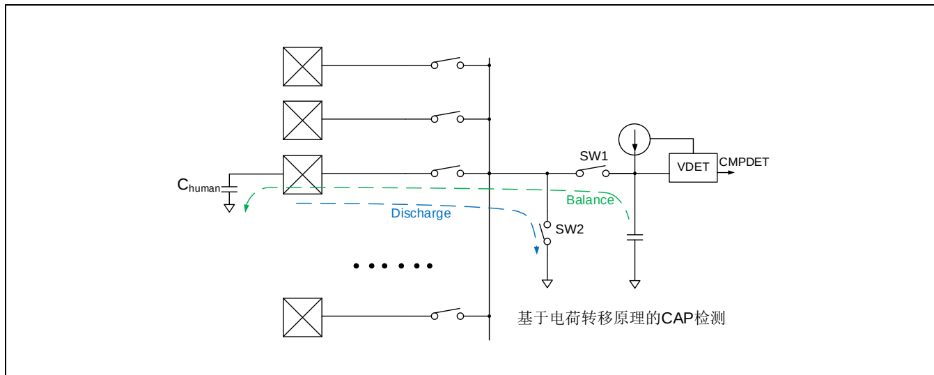
Figure 18-1 Touch Sensor模拟框图
