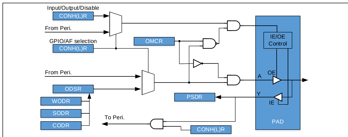
Figure 6-1 GPIO原理图
