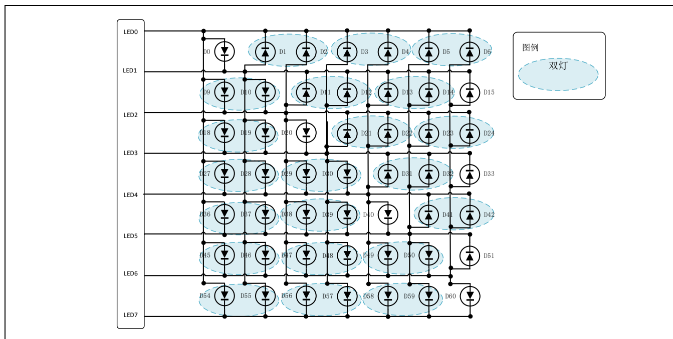
Figure 17-7 7*7点阵驱动
