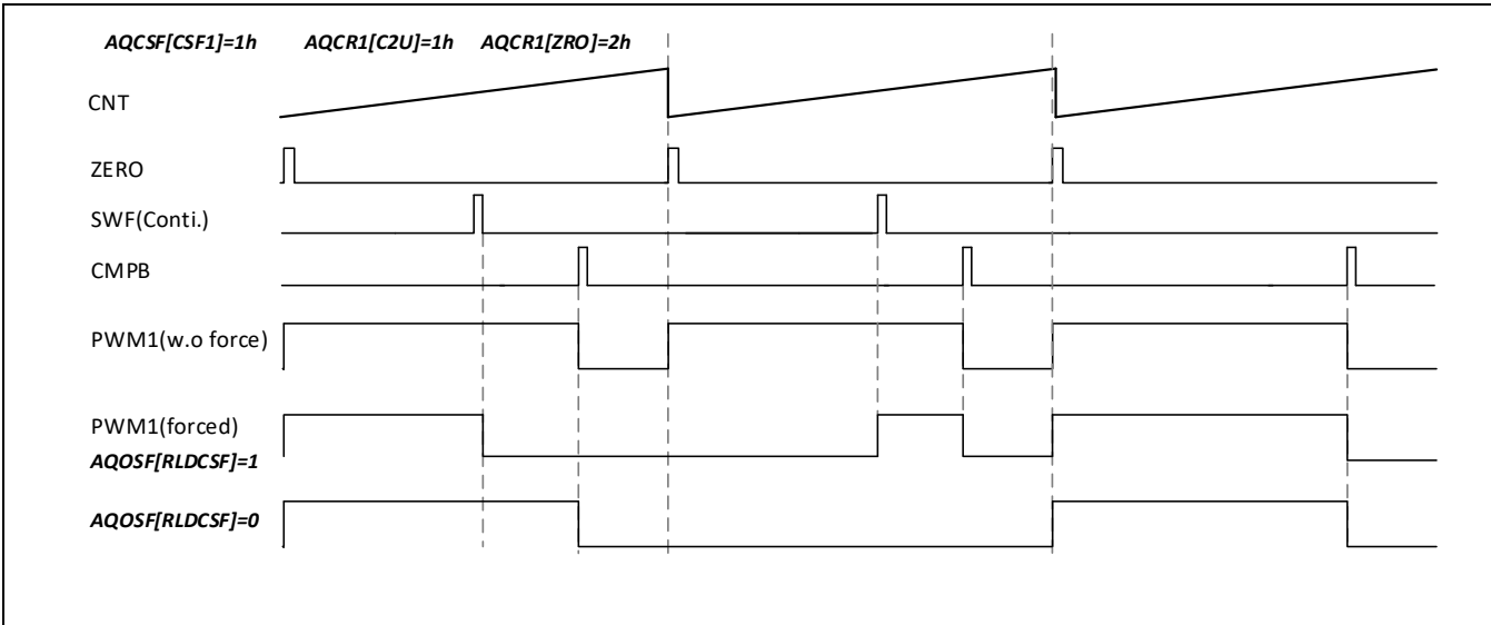
Figure 11-15 持续性软件强制输出
