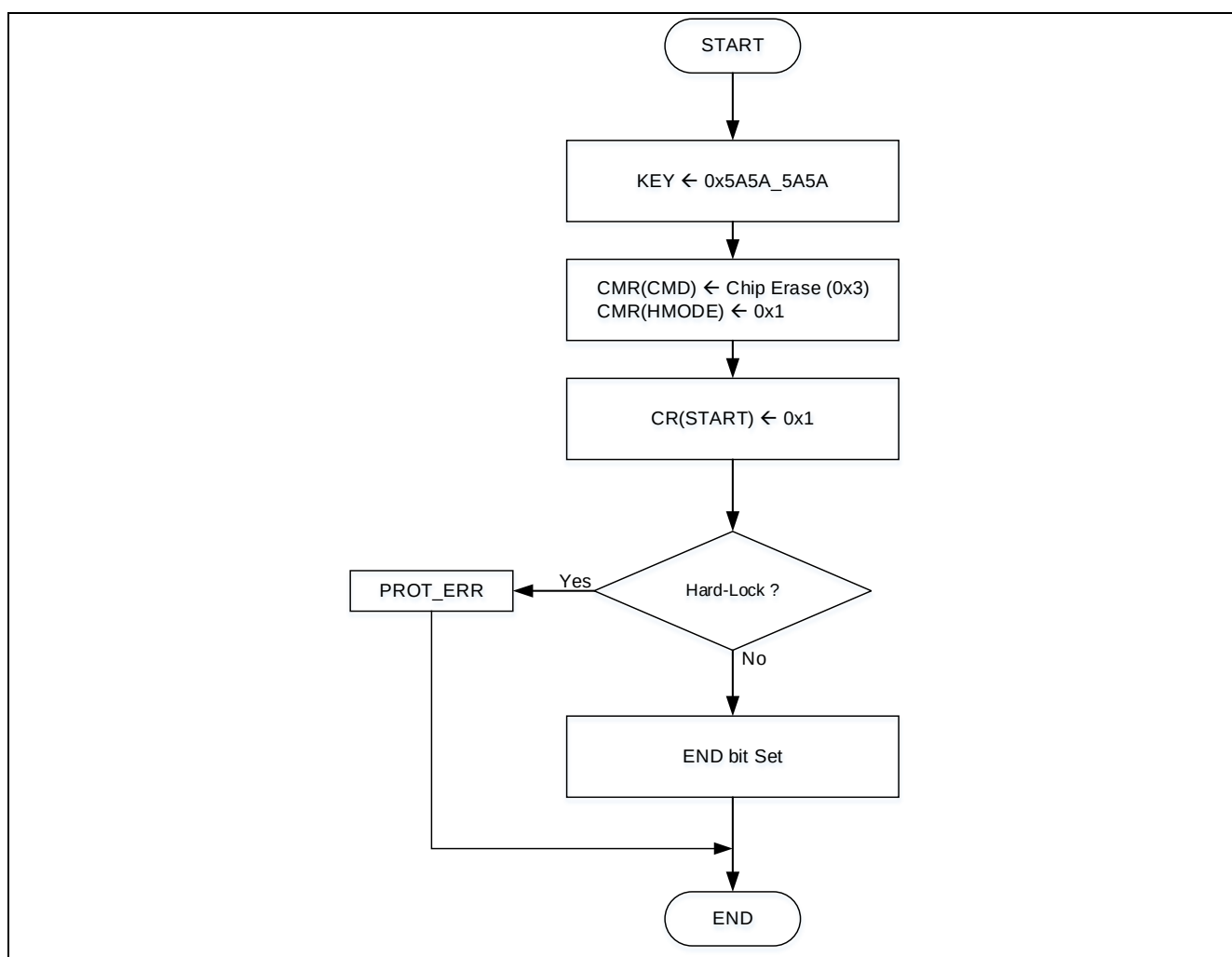
Figure 4-8 Chip Erase
