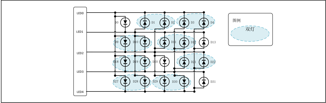
Figure 17-11 4*5点阵驱动
