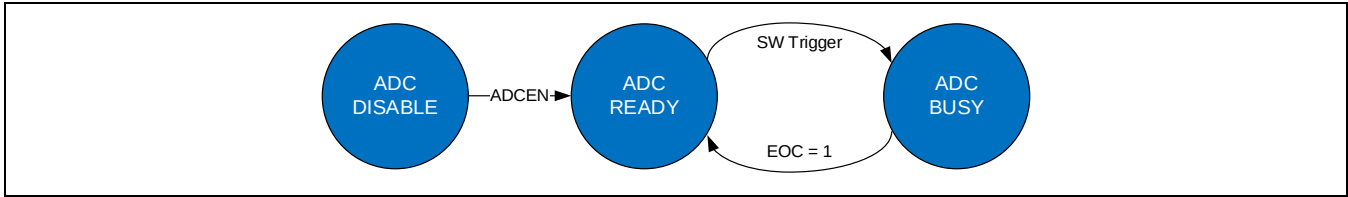
Figure 16-3 ADC状态机
