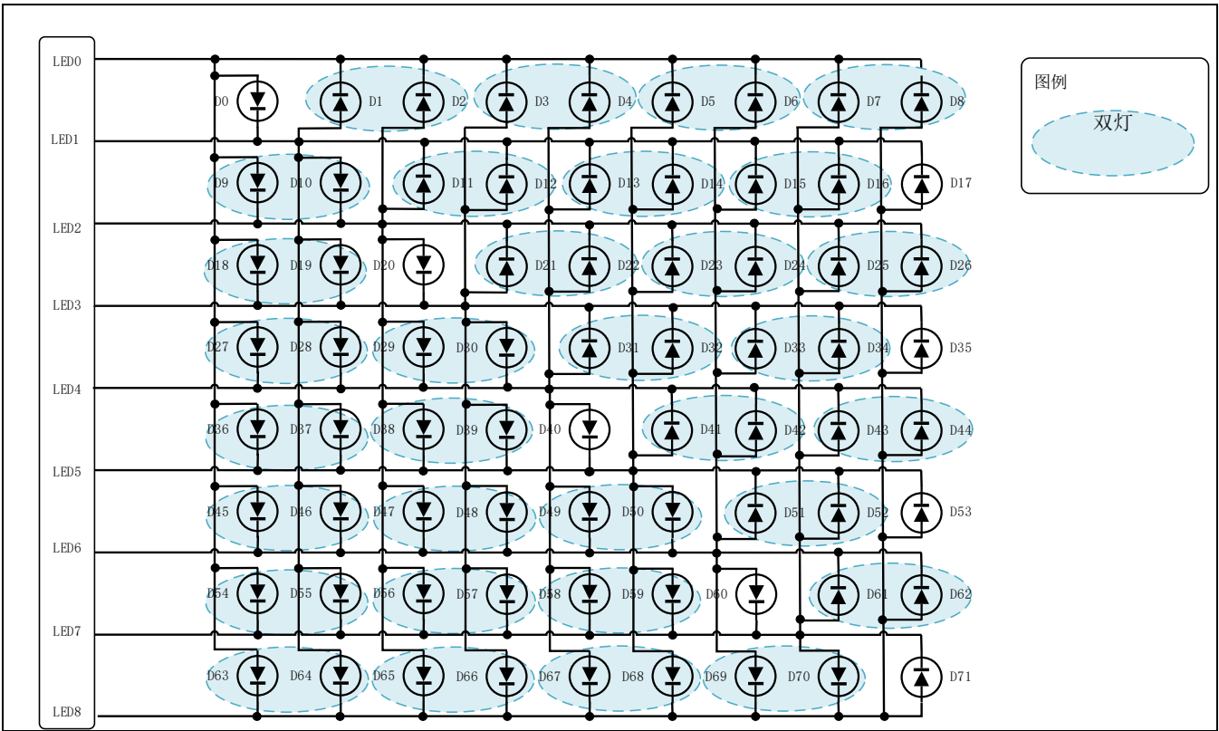
Figure 17-5 8*9点阵驱动
