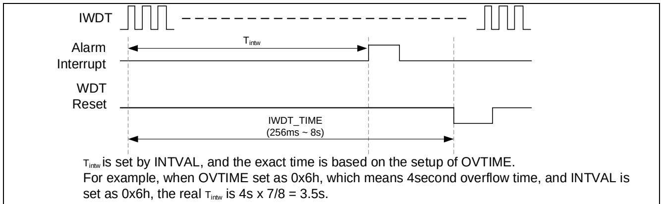
Figure 5-11 IWDT 计数器溢出和报警中断
