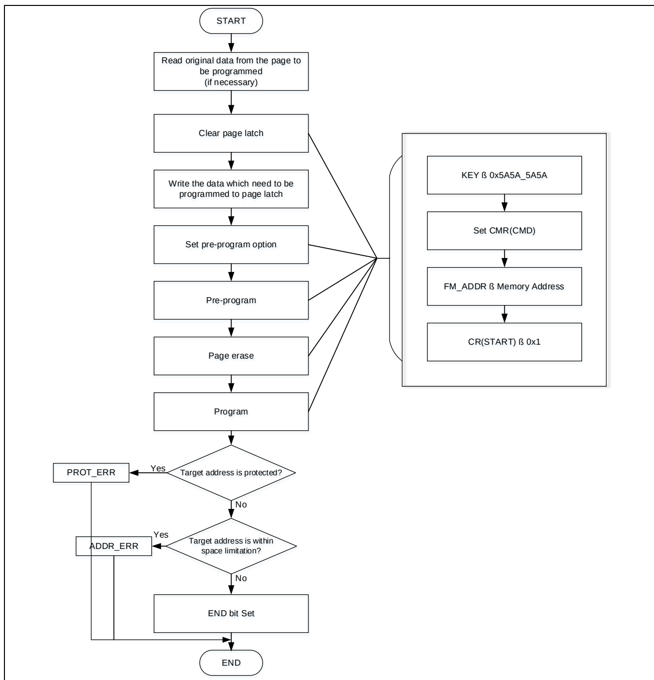
Figure 4-6 Flash Write – Parallel Mode
