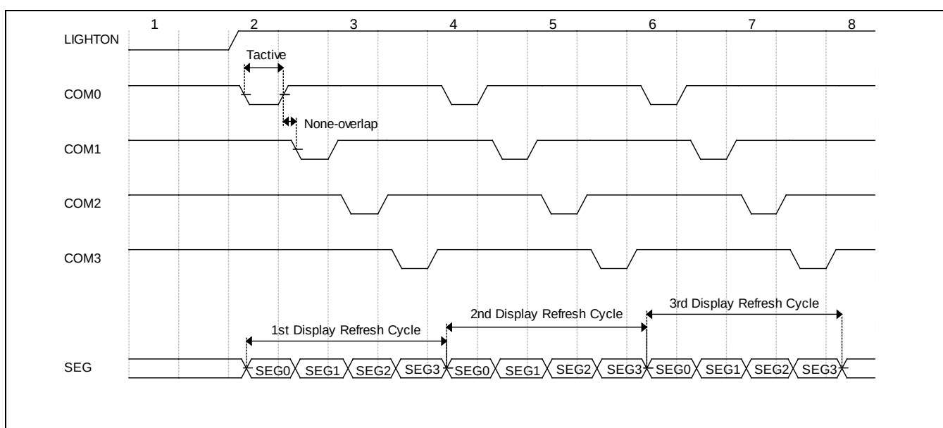
Figure 17-3 LED 扫描显示 (COM_EN = 8'b0000_1111模式)
