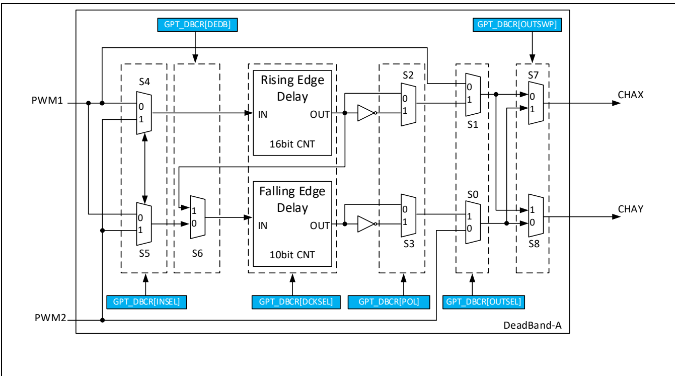
Figure 11-17 死区控制模块
