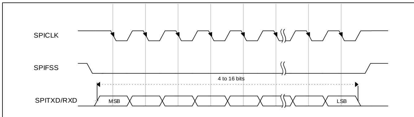
Figure 14-10 Motorola SPI 帧格式 (连续传输), SPO = 1 和 SPH = 0
