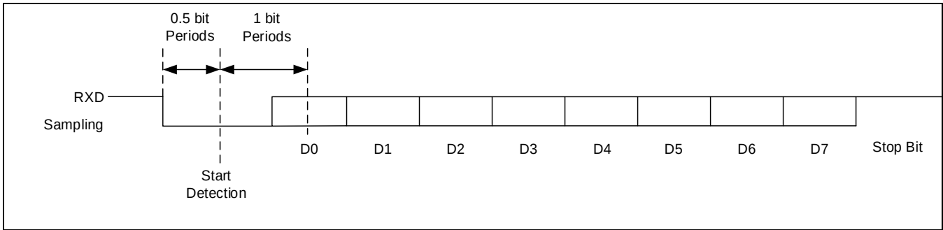
Figure 15-4 接收数据
