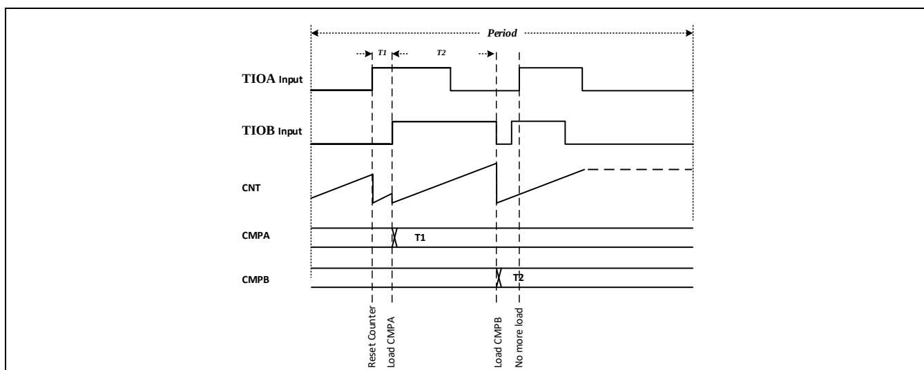
Figure 11-27 CHA的脉冲宽度检测
